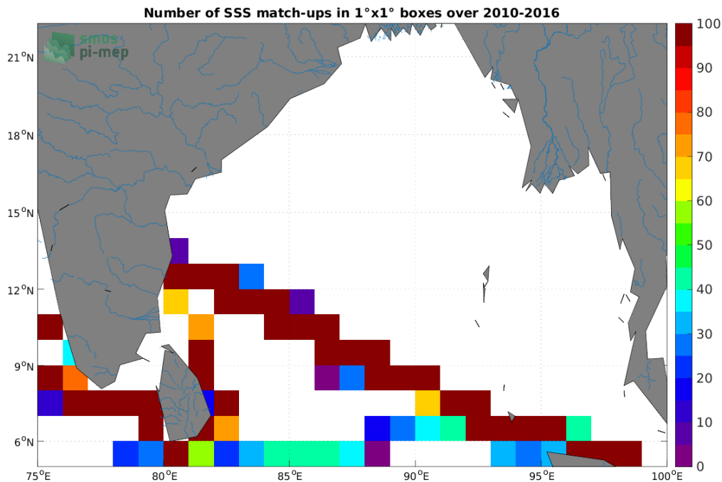
Figure 4: Number of SSS match-ups between TSG (LEGOS-DM) SSS and the SMOS SSS L4 v1 - Monthly (CMEMS-CNR) SSS product for the Ganga and Brahmaputra river plumes Pi-MEP region over 1°x1° boxes and for the full satellite product period.
