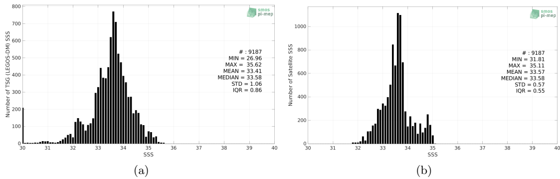
Figure 2: Histograms of SSS from TSG (LEGOS-DM) (a) and SMOS SSS L4 v1 - Monthly (CMEMS-CNR) (b) considering all match-up pairs per bins of 0.1 over the Ganga and Brahmaputra river plumes Pi-MEP region and for the full satellite product period.
