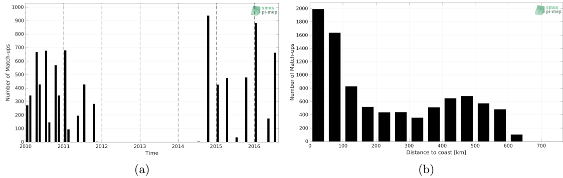
Figure 1: Number of match-ups between TSG (LEGOS-DM) and SMOS SSS L4 v1 - Monthly (CMEMS-CNR) SSS as a function of time (a) and as function of the distance to coast (b) over the Ganga and Brahmaputra river plumes Pi-MEP region and for the full satellite product period.
