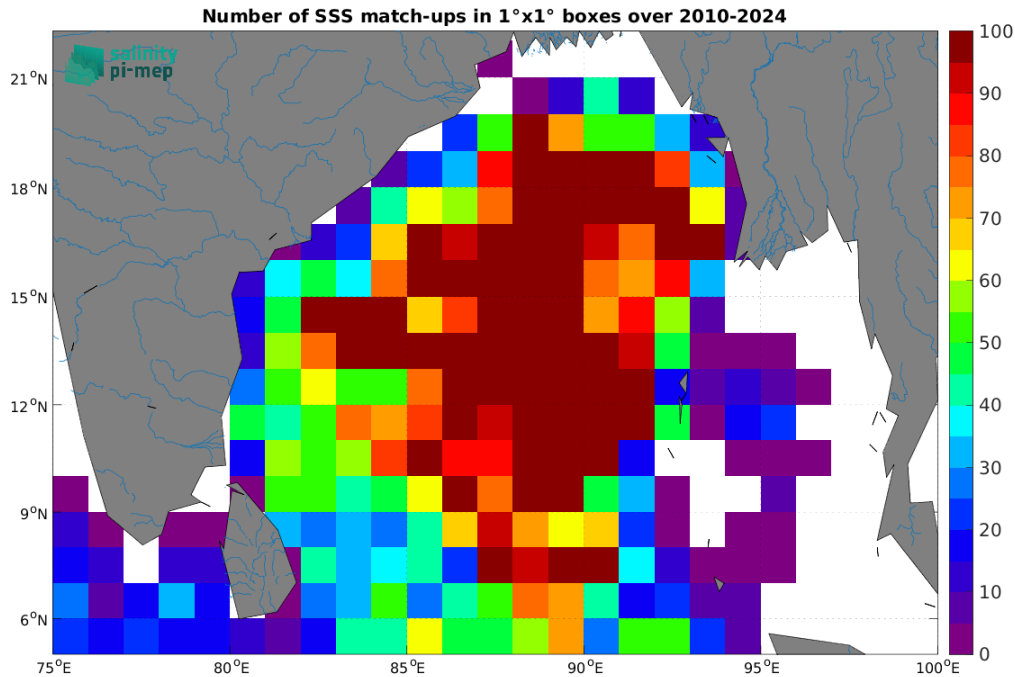
Figure 5: Number of SSS match-ups between Argo SSS and the SMOS SSS L4 v1 - Monthly (CMEMS-CNR) SSS product for the Ganga and Brahmaputra river plumes Pi-MEP region over 1^\circ \times 1^\circ boxes and for the full satellite product period.
