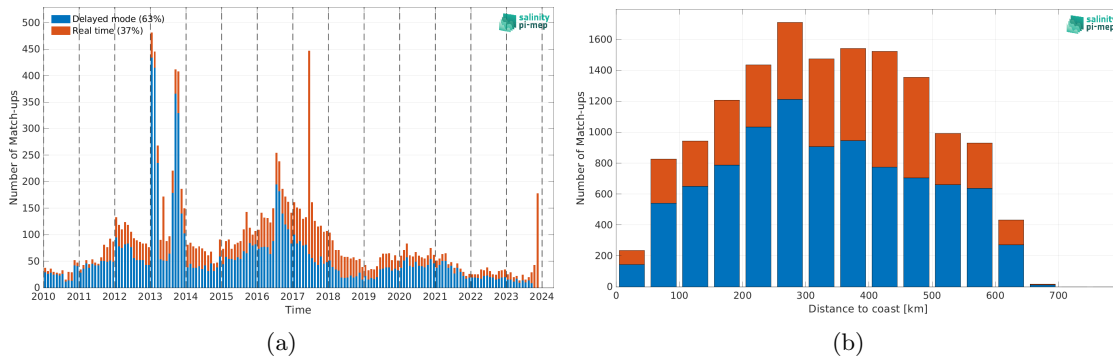
Figure 2: Number of match-ups between Argo and SMOS SSS L4 v1 - Monthly (CMEMS-CNR) SSS as a function of time (a) and as function of the distance to coast (b) over the Ganga and Brahmaputra river plumes Pi-MEP region and for the full satellite product period.
