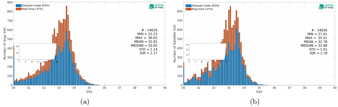
Figure 3: Histograms of SSS from Argo (a) and SMOS SSS L4 v1 - Monthly (CMEMS-CNR) (b) considering all match-up pairs per bins of 0.1 over the Ganga and Brahmaputra river plumes Pi-MEP region and for the full satellite product period.
