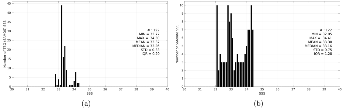
Figure 3: Histograms of SSS from TSG (SAMOS) (a) and SMOS SSS L4 v2 - Daily (BEC) (b) considering all match-up pairs per bins of 0.1 over the Ganga and Brahmaputra river plumes Pi-MEP region and for the full satellite product period.
