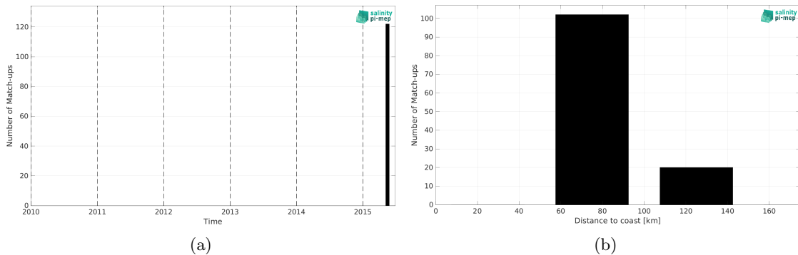
Figure 2: Number of match-ups between TSG (SAMOS) and SMOS SSS L4 v2 - Daily (BEC) SSS as a function of time (a) and as function of the distance to coast (b) over the Ganga and Brahmaputra river plumes Pi-MEP region and for the full satellite product period.
