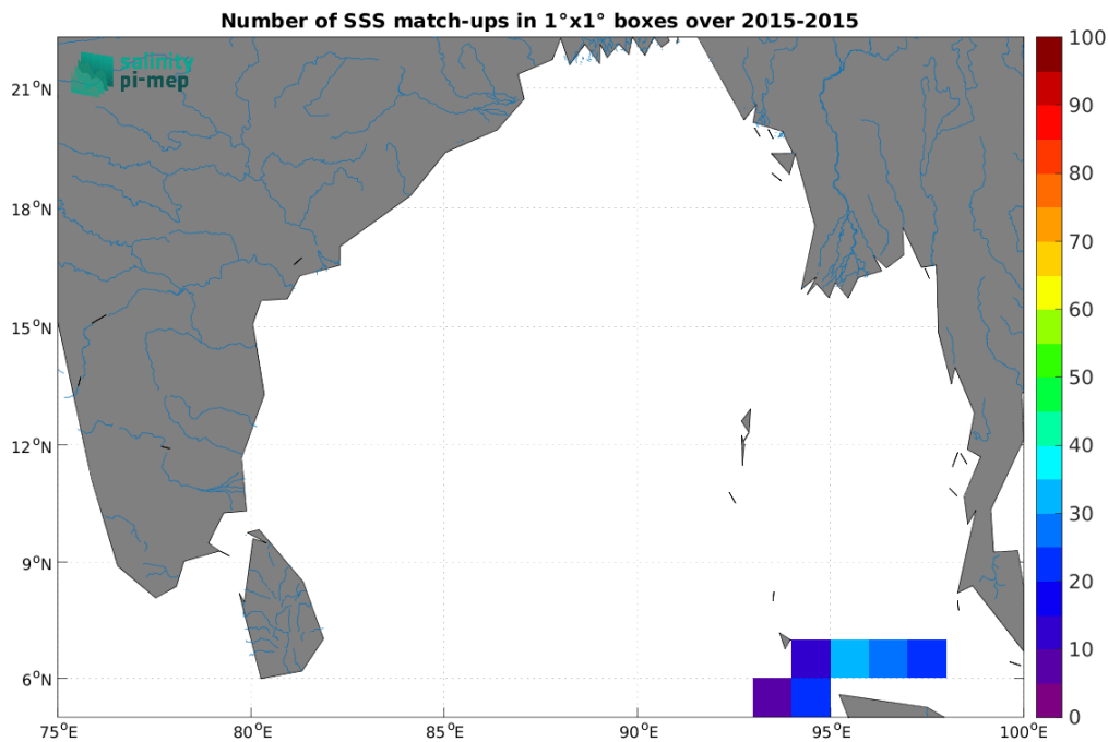
Figure 5: Number of SSS match-ups between TSG (SAMOS) SSS and the SMOS SSS L4 v2 - Daily (BEC) SSS product for the Ganga and Brahmaputra river plumes Pi-MEP region over 1^\circ \times 1^\circ boxes and for the full satellite product period.
