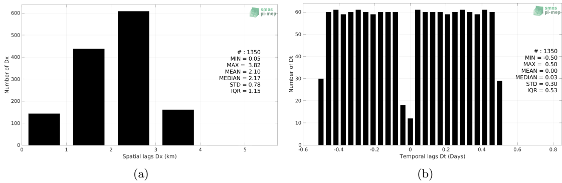
Figure 5: Histograms of the spatial (a) and temporal (b) lags between the location/time of the TSG (SAMOS) measurement and the date of the corresponding SMOS SSS L4 v2 - Daily (BEC) SSS pixel.
