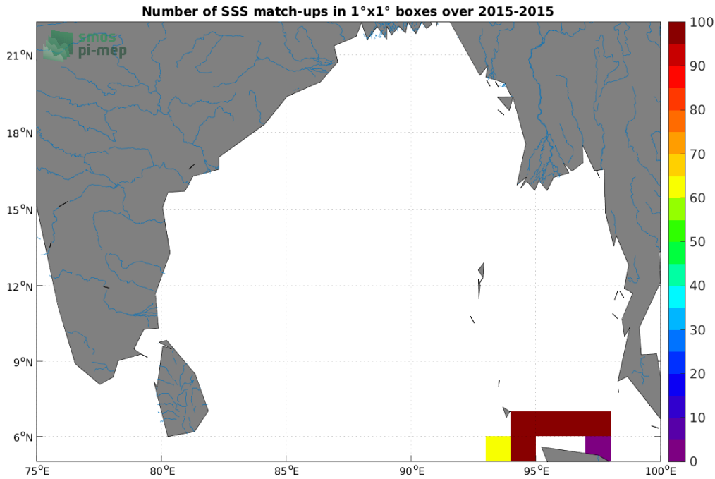
Figure 4: Number of SSS match-ups between TSG (SAMOS) SSS and the SMOS SSS L4 v2 - Daily (BEC) SSS product for the Ganga and Brahmaputra river plumes Pi-MEP region over 1^\circ \times 1^\circ boxes and for the full satellite product period.
