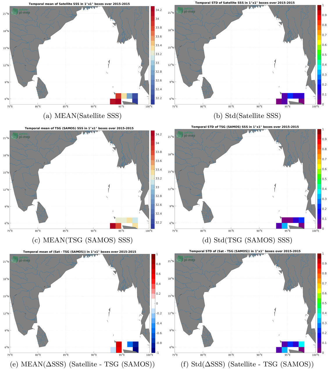
Figure 6: Temporal mean (left) and Std (right) of SSS from SMOS SSS L4 v2 - Daily (BEC) (top), TSG (SAMOS) (middle), and of \Delta SSS (Satellite - TSG (SAMOS)). Only match-up pairs are used to generate these maps.
