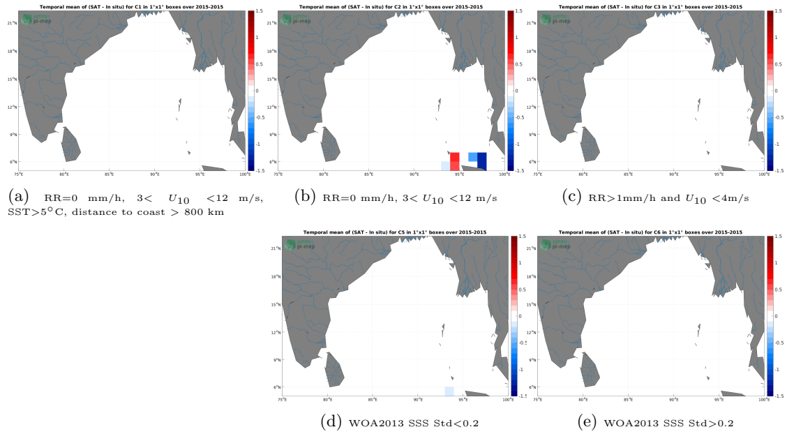
Figure 12: Temporal mean gridded over spatial boxes of size 1^\circ \times 1^\circ of \Delta SSS (SMOS SSS L4 v2 - Daily (BEC) - TSG (SAMOS)) for 5 different subdatasets corresponding to:RR=0 mm/h, 3 < U_{10} < 12 m/s, SST >5^\circ C, distance to coast > 800 km (a), RR=0 mm/h, 3 < U_{10} < 12 m/s (b), RR >1 mm/h and U_{10} < 4 m/s (c), WOA2013 SSS Std <0.2 (d), WOA2013 SSS Std >0.2 (e).
