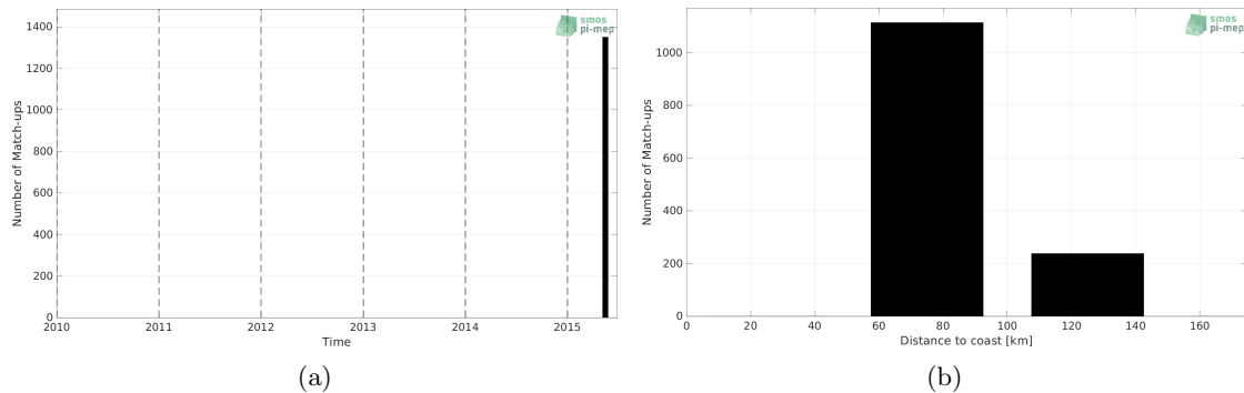
Figure 1: Number of match-ups between TSG (SAMOS) and SMOS SSS L4 v2 - Daily (BEC) SSS as a function of time (a) and as function of the distance to coast (b) over the Ganga and Brahmaputra river plumes Pi-MEP region and for the full satellite product period.
