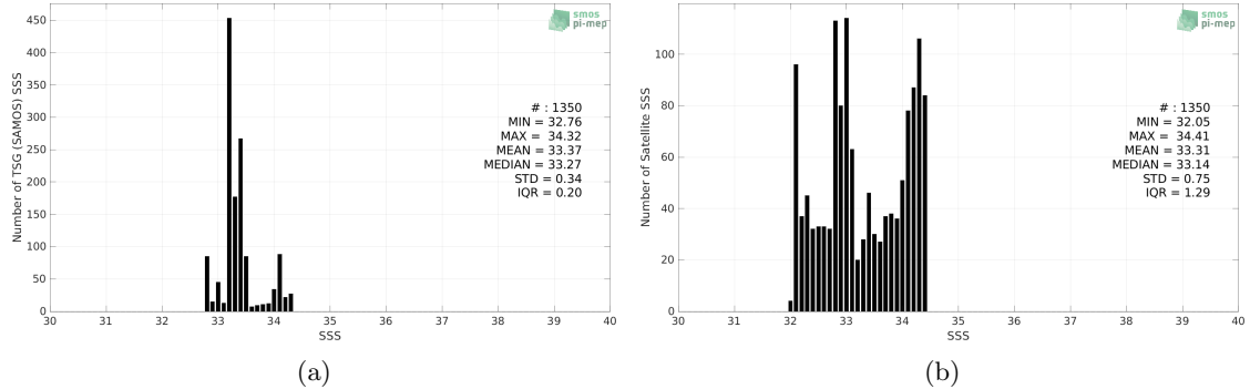
Figure 2: Histograms of SSS from TSG (SAMOS) (a) and SMOS SSS L4 v2 - Daily (BEC) (b) considering all match-up pairs per bins of 0.1 over the Ganga and Brahmaputra river plumes Pi-MEP region and for the full satellite product period.
