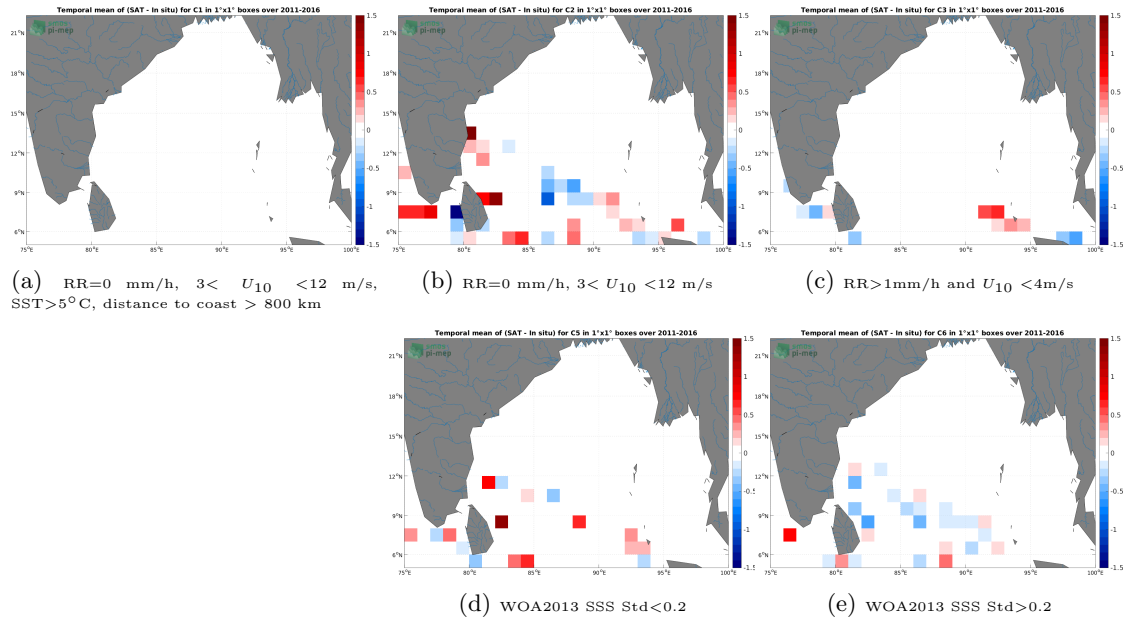
Figure 12: Temporal mean gridded over spatial boxes of size 1^\circ \times 1^\circ of \Delta SSS (SMOS SSS L4 v2 - Daily (BEC) - TSG (LEGOS-DM)) for 5 different subdatasets corresponding to:RR=0 mm/h, 3 < U_{10} < 12 m/s, SST >5^\circ C, distance to coast > 800 km (a), RR=0 mm/h, 3 < U_{10} < 12 m/s (b), RR >1 mm/h and U_{10} < 4 m/s (c), WOA2013 SSS Std <0.2 (d), WOA2013 SSS Std >0.2 (e).
