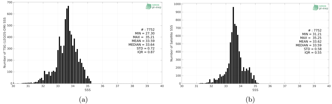
Figure 2: Histograms of SSS from TSG (LEGOS-DM) (a) and SMOS SSS L4 v2 - Daily (BEC) (b) considering all match-up pairs per bins of 0.1 over the Ganga and Brahmaputra river plumes Pi-MEP region and for the full satellite product period.
