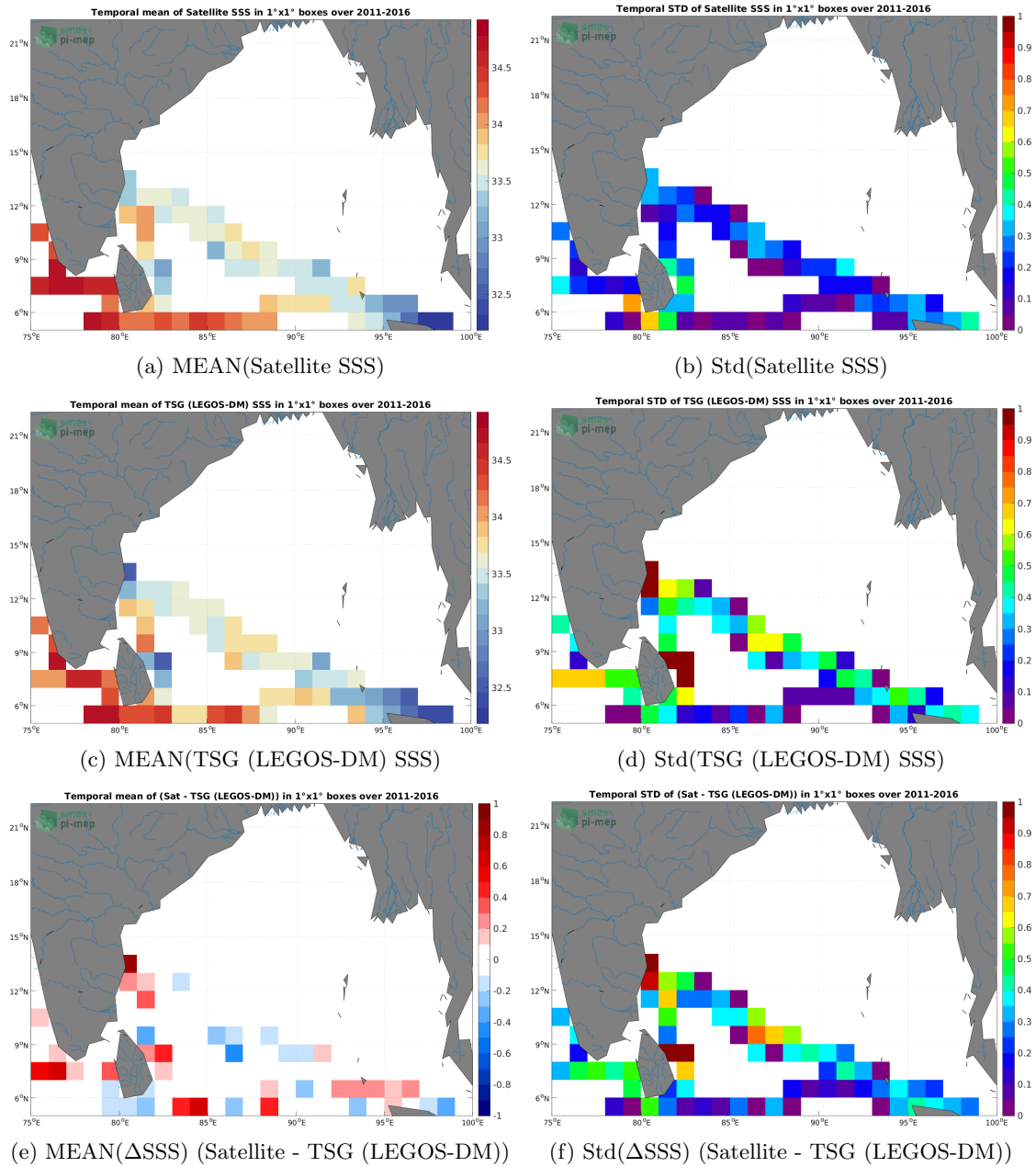
Figure 6: Temporal mean (left) and Std (right) of SSS from SMOS SSS L4 v2 - Daily (BEC) (top), TSG (LEGOS-DM) (middle), and of \Delta SSS (Satellite - TSG (LEGOS-DM)). Only match-pairs are used to generate these maps.
