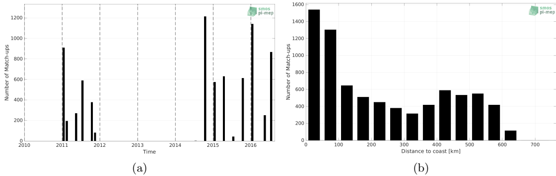
Figure 1: Number of match-ups between TSG (LEGOS-DM) and SMOS SSS L4 v2 - Daily (BEC) SSS as a function of time (a) and as function of the distance to coast (b) over the Ganga and Brahmaputra river plumes Pi-MEP region and for the full satellite product period.
