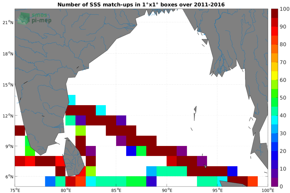
Figure 4: Number of SSS match-ups between TSG (LEGOS-DM) SSS and the SMOS SSS L4 v2 - Daily (BEC) SSS product for the Ganga and Brahmaputra river plumes Pi-MEP region over 1°×1° boxes and for the full satellite product period.
