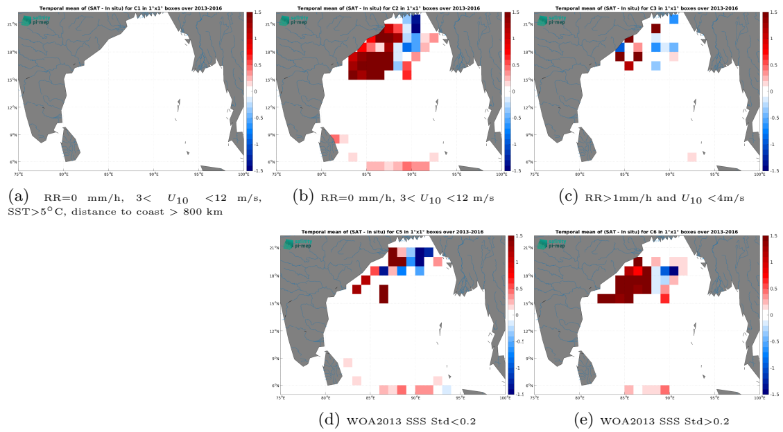
Figure 11: Temporal mean gridded over spatial boxes of size 1^\circ \times 1^\circ of \Delta SSS (SMOS SSS L4 v2 - Daily (BEC) - Surface drifters) for 5 different subdatasets corresponding to:RR=0 mm/h, 3 < U_{10} < 12 m/s, SST >5^\circ C, distance to coast > 800 km (a), RR=0 mm/h, 3 < U_{10} < 12 m/s (b), RR >1 mm/h and U_{10} < 4 m/s (c), WOA2013 SSS Std <0.2 (d), WOA2013 SSS Std >0.2 (e).
