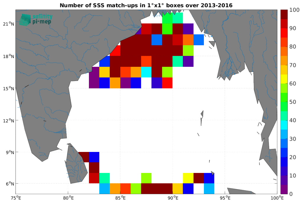
Figure 3: Number of SSS match-ups between Surface drifters SSS and the SMOS SSS L4 v2 - Daily (BEC) SSS product for the Ganga and Brahmaputra river plumes Pi-MEP region over 1^\circ \times 1^\circ boxes and for the full satellite product period.
