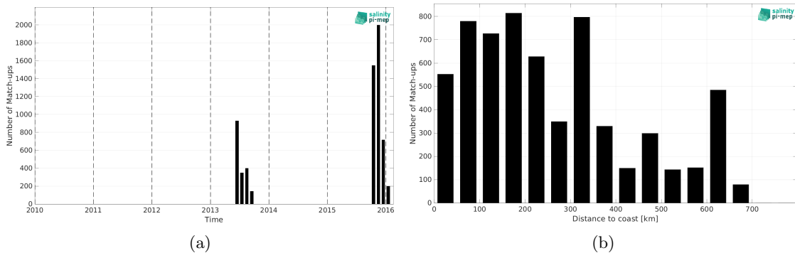
Figure 1: Number of match-ups between Surface drifters and SMOS SSS L4 v2 - Daily (BEC) SSS as a function of time (a) and as function of the distance to coast (b) over the Ganga and Brahmaputra river plumes Pi-MEP region and for the full satellite product period.
