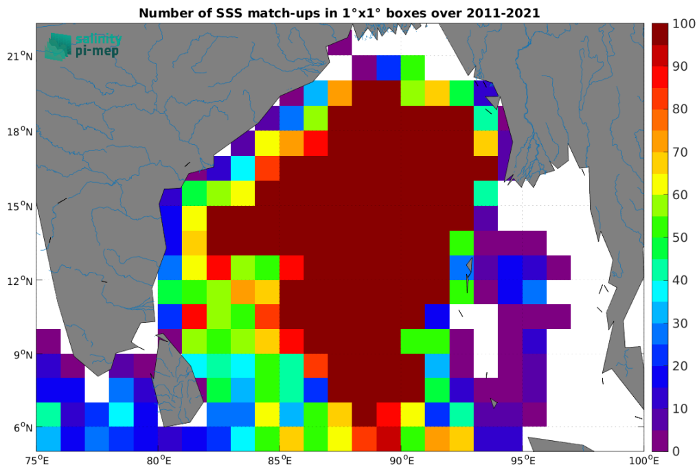
Figure 5: Number of SSS match-ups between Argo SSS and the SMOS SSS L4 v2 - Daily (BEC) SSS product for the Ganga and Brahmaputra river plumes Pi-MEP region over 1^\circ \times 1^\circ boxes and for the full satellite product period.
