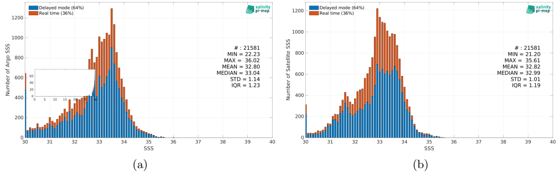
Figure 2: Histograms of SSS from Argo (a) and SMOS SSS L4 v2 - Daily (BEC) (b) considering all match-up pairs per bins of 0.1 over the Ganga and Brahmaputra river plumes Pi-MEP region and for the full satellite product period.
