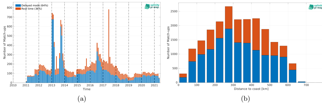
Figure 1: Number of match-ups between Argo and SMOS SSS L4 v2 - Daily (BEC) SSS as a function of time (a) and as function of the distance to coast (b) over the Ganga and Brahmaputra river plumes Pi-MEP region and for the full satellite product period.
