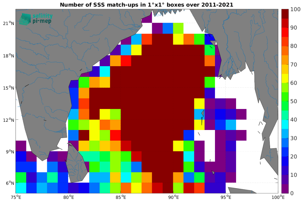
Figure 4: Number of SSS match-ups between Argo SSS and the SMOS SSS L4 v2 - Daily (BEC) SSS product for the Ganga and Brahmaputra river plumes Pi-MEP region over 1^\circ \times 1^\circ boxes and for the full satellite product period.
