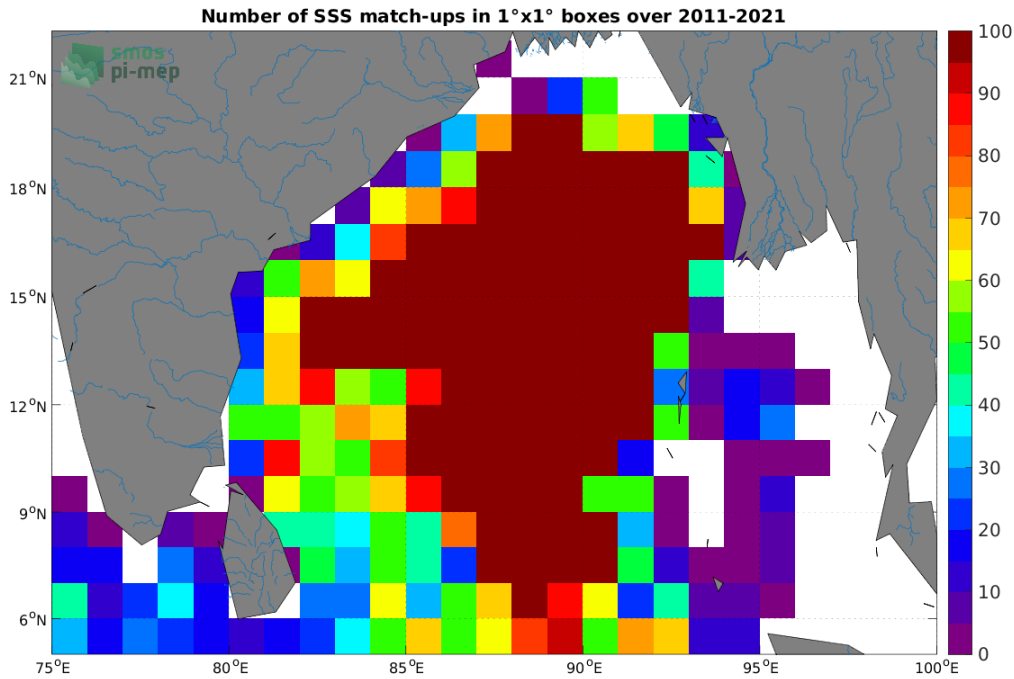
Figure 4: Number of SSS match-ups between Argo SSS and the SMOS SSS L4 v2 - Daily (BEC) SSS product for the Ganga and Brahmaputra river plumes Pi-MEP region over 1^{\circ} \times 1^{\circ} boxes and for the full satellite product period.
