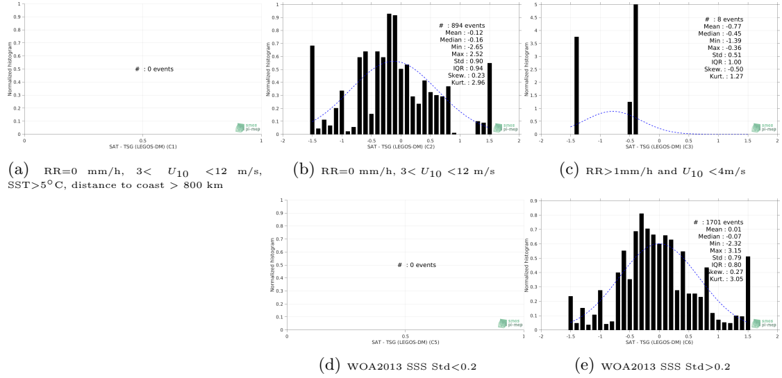
Figure 13: Normalized histogram of \Delta\text{SSS} (SMOS SSS L3 v3 Monthly (ICDC) - TSG (LEGOS-DM)) for 5 different subdatasets corresponding to: RR=0 mm/h, 3 < U_{10} < 12 m/s, SST > 5^{\circ}\text{C} , distance to coast > 800 km (a), RR=0 mm/h, 3 < U_{10} < 12 m/s (b), RR > 1\text{mm/h} and U_{10} < 4\text{m/s} (c), WOA2013 SSS Std < 0.2 (d), WOA2013 SSS Std > 0.2 (e).
