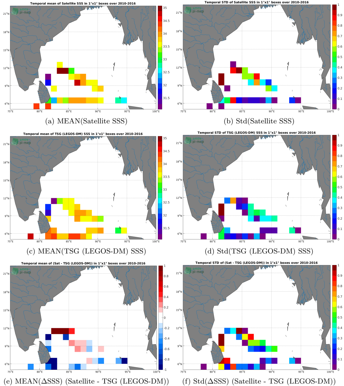
Figure 6: Temporal mean (left) and Std (right) of SSS from SMOS SSS L3 v3 Monthly (ICDC) (top), TSG (LEGOS-DM) (middle), and of \Delta SSS (Satellite - TSG (LEGOS-DM)). Only match-pairs are used to generate these maps.
