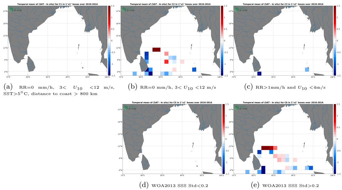
Figure 12: Temporal mean gridded over spatial boxes of size 1°x1° of \Delta SSS (SMOS SSS L3 v3 Monthly (ICDC) - TSG (LEGOS-DM)) for 5 different subdatasets corresponding to:RR=0 mm/h, 3 < U_{10} < 12 m/s, SST>5°C, distance to coast > 800 km (a), RR=0 mm/h, 3 < U_{10} < 12 m/s (b), RR>1mm/h and U_{10} < 4 m/s (c), WOA2013 SSS Std<0.2 (d), WOA2013 SSS Std>0.2 (e).
