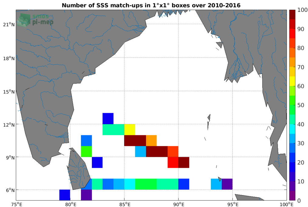
Figure 4: Number of SSS match-ups between TSG (LEGOS-DM) SSS and the SMOS SSS L3 v3 Monthly (ICDC) SSS product for the Ganga and Brahmaputra river plumes Pi-MEP region over 1°x1° boxes and for the full satellite product period.
