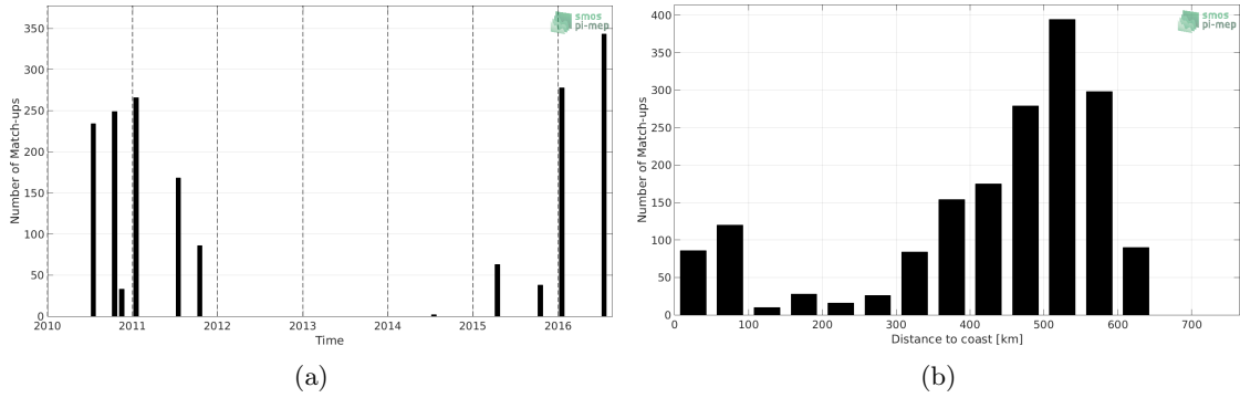
Figure 1: Number of match-ups between TSG-LEGOS-DM and SMOS-L3-ICDC-V3-MONTHLY-0.5DEG SSS as a function of time (a) and as function of the distance to coast (b) over the Ganga and Brahmaputra river plumes Pi-MEP region and for the full satellite product period.
