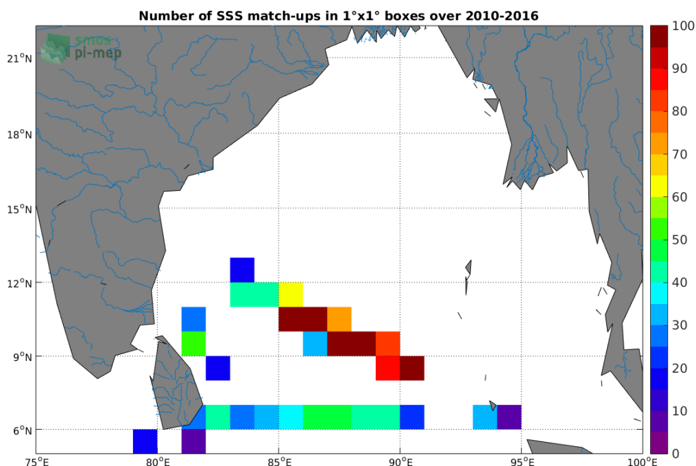
Figure 4: Number of SSS match-ups between TSG-LEGOS-DM SSS and the SMOS-L3-ICDC-V3-MONTHLY-0.5DEG SSS product for the Ganga and Brahmaputra river plumes Pi-MEP region over 1°x1° boxes and for the full satellite product period.
