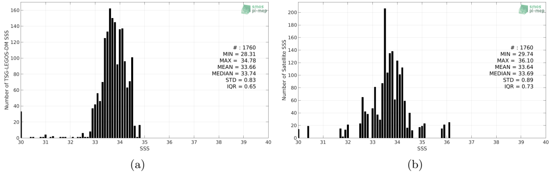
Figure 2: Histograms of SSS from TSG-LEGOS-DM (a) and SMOS-L3-ICDC-V3-MONTHLY-0.5DEG (b) considering all match-up pairs per bins of 0.1 over the Ganga and Brahmaputra river plumes Pi-MEP region and for the full satellite product period.
