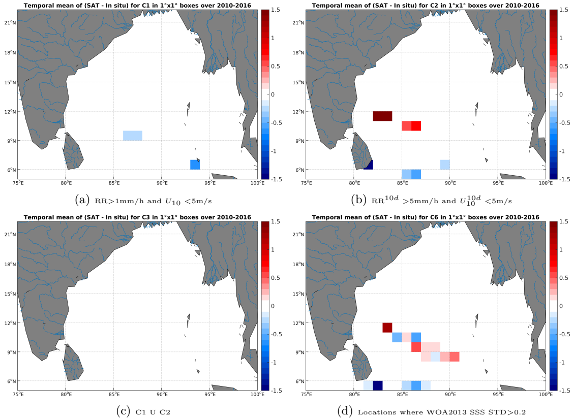
Figure 12: Temporal mean gridded over spatial boxes of size 1°x1° of \Delta SSS (SMOS-L3-ICDC-V3-MONTHLY-0.5DEG - TSG-LEGOS-DM) for 4 different subdatasets corresponding to: RR > 1mm/h and U_{10} < 5 m/s (a), RR^{10d} > 5 mm/h and U_{10}^{10d} < 5 m/s (b), C1 U C2 (c), Locations where WOA2013 SSS STD > 0.2 (d).
