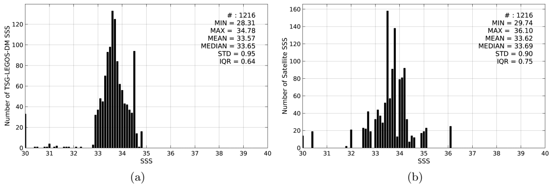
Figure 2: Histograms of SSS from TSG-LEGOS-DM (a) and SMOS-L3-ICDC-V3-MONTHLY-0.5DEG (b) considering all match-up pairs per bins of 0.1 over the Ganga and Brahmaputra river plumes Pi-MEP region and for the full satellite product period.
