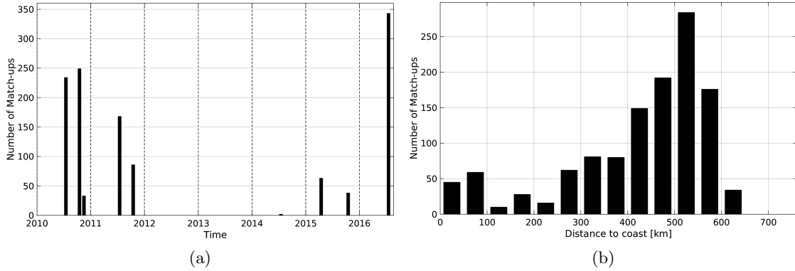
Figure 1: Number of match-ups between TSG-LEGOS-DM and SMOS-L3-ICDC-V3-MONTHLY-0.5DEG SSS as a function of time (a) and as function of the distance to coast (b) over the Ganga and Brahmaputra river plumes Pi-MEP region and for the full satellite product period.
