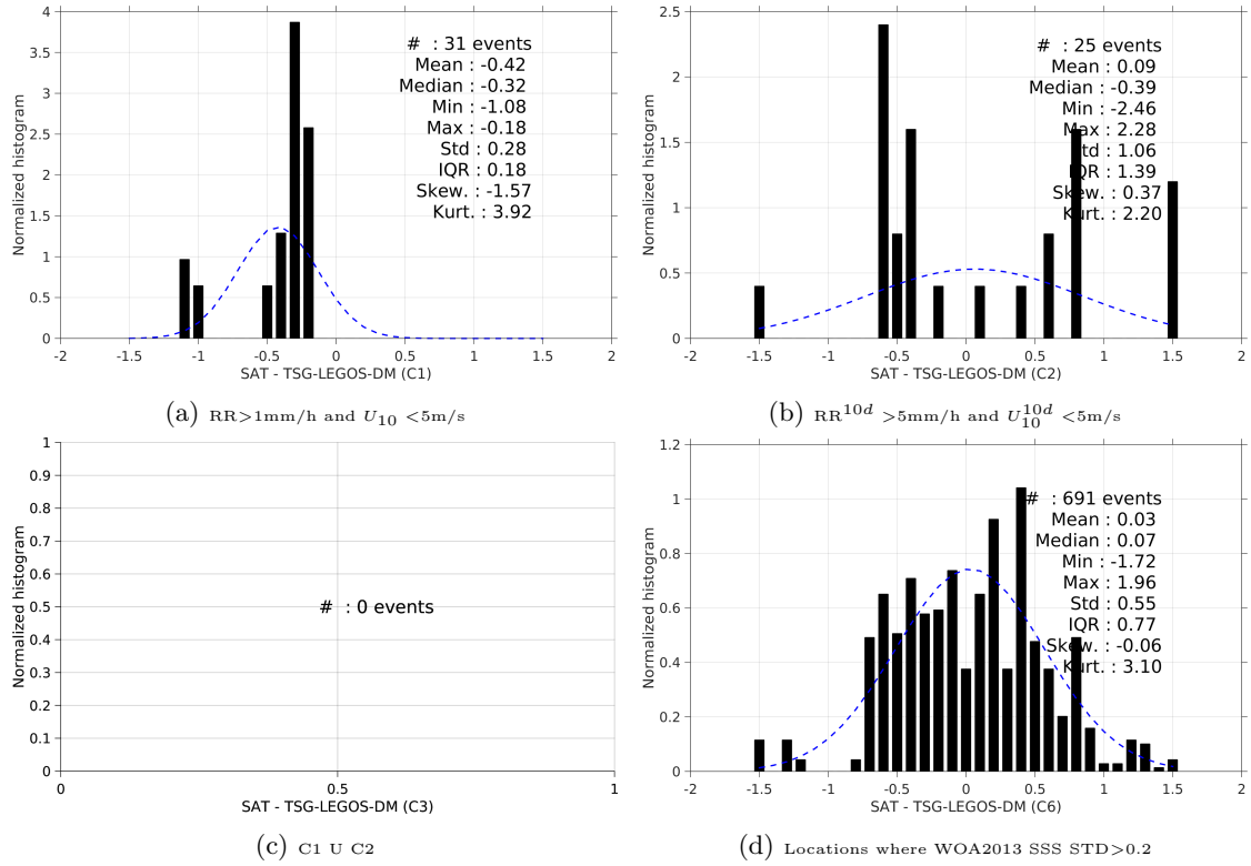
Figure 13: Normalized histogram of \Delta\text{SSS} (SMOS-L3-ICDC-V3-MONTHLY-0.5DEG - TSG-LEGOS-DM) for 6 different subdatasets corresponding to: RR>1mm/h and U_{10} < 5\text{m/s} (a), \text{RR}^{10d} > 5\text{mm/h} and U_{10}^{10d} < 5\text{m/s} (b), C1 U C2 (c), Locations where WOA2013 SSS STD>0.2 (d).
