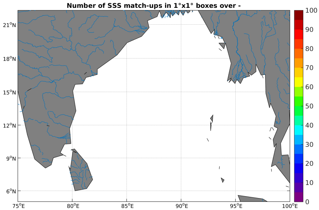
Figure 4: Number of SSS match-ups between TSG-GOSUD-Sailing-ship SSS and the SMOS-L3-ICDC-V3-MONTHLY-0.5DEG SSS product for the Ganga and Brahmaputra river plumes Pi-MEP region over 1^\circ \times 1^\circ boxes and for the full satellite product period.
