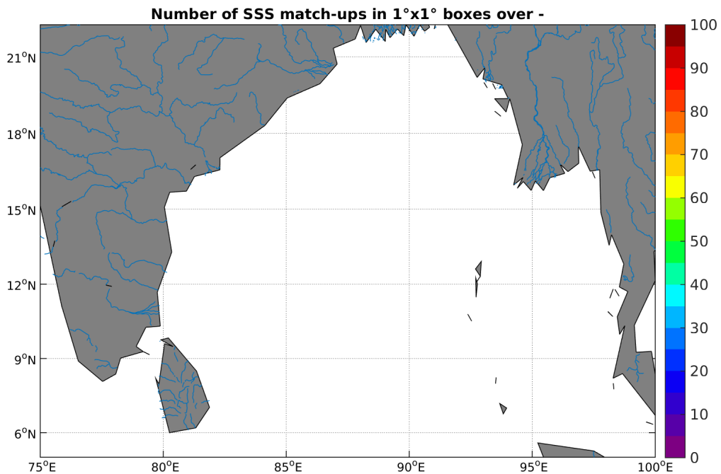
Figure 4: Number of SSS match-ups between TSG-GOSUD-Research-vessel SSS and the SMOS-L3-ICDC-V3-MONTHLY-0.5DEG SSS product for the Ganga and Brahmaputra river plumes Pi-MEP region over 1°x1° boxes and for the full satellite product period.
