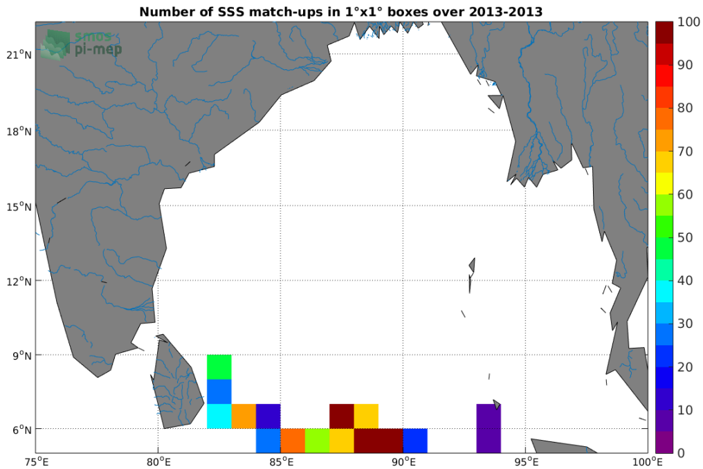
Figure 3: Number of SSS match-ups between Surface drifters SSS and the SMOS-L3-ICDC-V3-MONTHLY-0.5DEG SSS product for the Ganga and Brahmaputra river plumes Pi-MEP region over 1^{\circ} \times 1^{\circ} boxes and for the full satellite product period.
