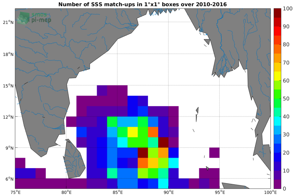
Figure 4: Number of SSS match-ups between Argo SSS and the SMOS SSS L3 v3 Monthly (ICDC) SSS product for the Ganga and Brahmaputra river plumes Pi-MEP region over 1^{\circ} \times 1^{\circ} boxes and for the full satellite product period.
