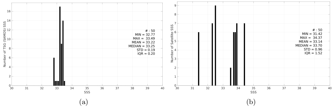
Figure 3: Histograms of SSS from TSG (SAMOS) (a) and SMOS SSS L2Q v331 - With FLAG (CMEMS-CATDS-CPDC) (b) considering all match-up pairs per bins of 0.1 over the Ganga and Brahmaputra river plumes Pi-MEP region and for the full satellite product period.
