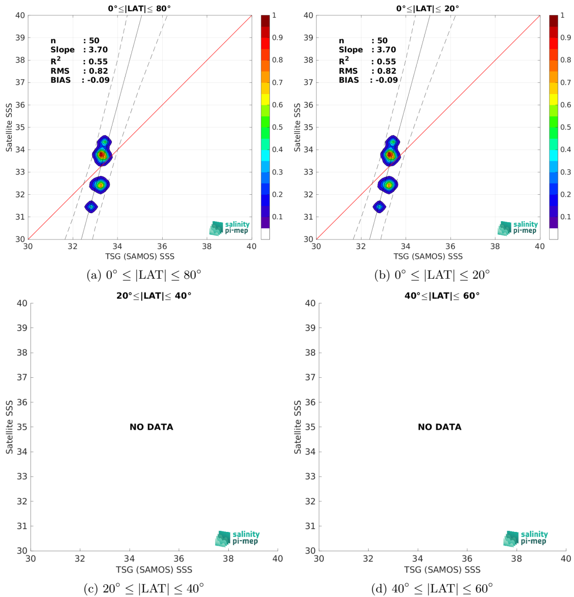
Figure 10: Contour maps of the concentration of SMOS SSS L2Q v331 - With FLAG (CMEMS-CATDS-CPDC) SSS (y-axis) versus TSG (SAMOS) SSS (x-axis) at match-up pairs for different latitude bands. For each plot, the red line shows x=y . The black thin and dashed lines indicate a linear fit through the data cloud and the \pm 95\% confidence levels, respectively. The number match-up pairs n , the slope and R^2 coefficient of the linear fit, the root mean square (RMS) and the mean bias between satellite and in situ data are indicated for each latitude band in each plots.
