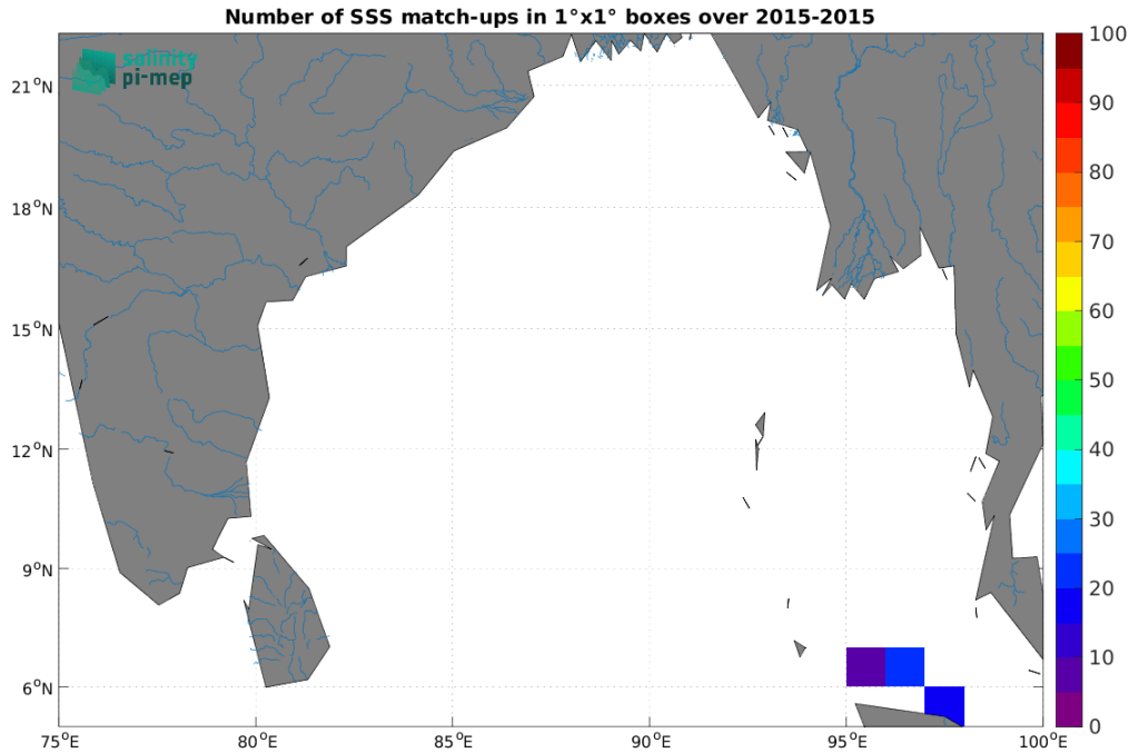
Figure 5: Number of SSS match-ups between TSG (SAMOS) SSS and the SMOS SSS L2Q v331 - With FLAG (CMEMS-CATDS-CPDC) SSS product for the Ganga and Brahmaputra river plumes Pi-MEP region over 1^\circ \times 1^\circ boxes and for the full satellite product period.
