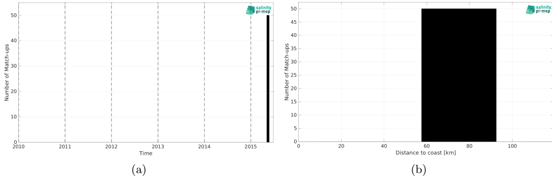
Figure 2: Number of match-ups between TSG (SAMOS) and SMOS SSS L2Q v331 - With FLAG (CMEMS-CATDS-CPDC) SSS as a function of time (a) and as function of the distance to coast (b) over the Ganga and Brahmaputra river plumes Pi-MEP region and for the full satellite product period.
