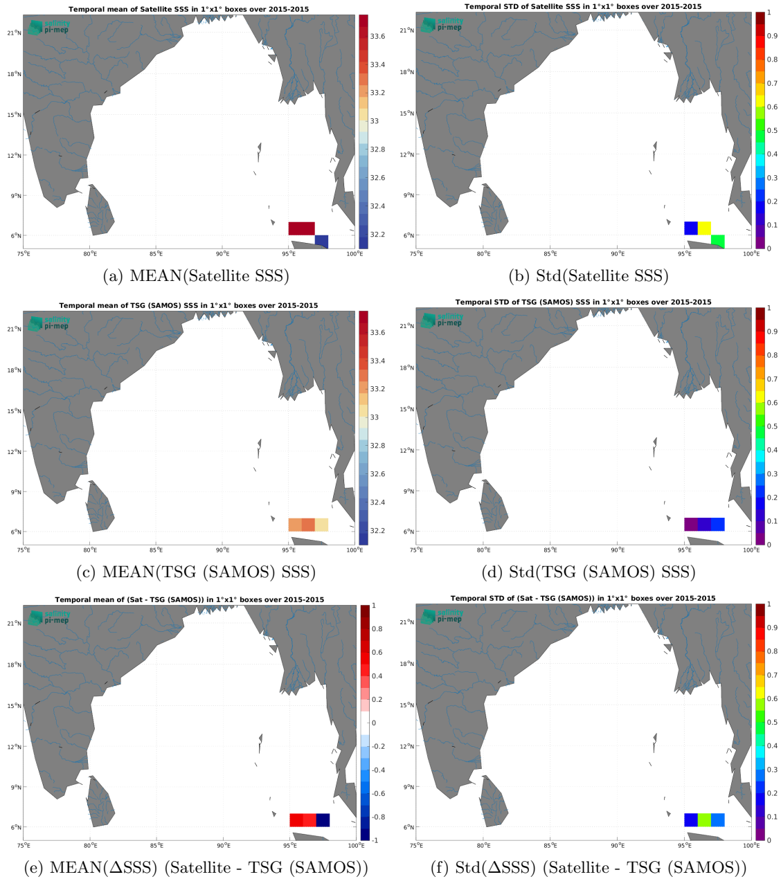
Figure 7: Temporal mean (left) and Std (right) of SSS from SMOS SSS L2Q v331 - With FLAG (CMEMS-CATDS-CPDC) (top), TSG (SAMOS) (middle), and of \Delta SSS (Satellite - TSG (SAMOS)). Only match-up pairs are used to generate these maps.
