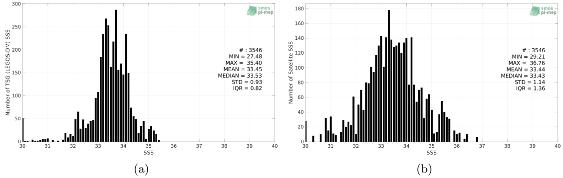
Figure 2: Histograms of SSS from TSG (LEGOS-DM) (a) and SMOS SSS L2Q v331 - With FLAG (CMEMS-CATDS-CPDC) (b) considering all match-up pairs per bins of 0.1 over the Ganga and Brahmaputra river plumes Pi-MEP region and for the full satellite product period.
