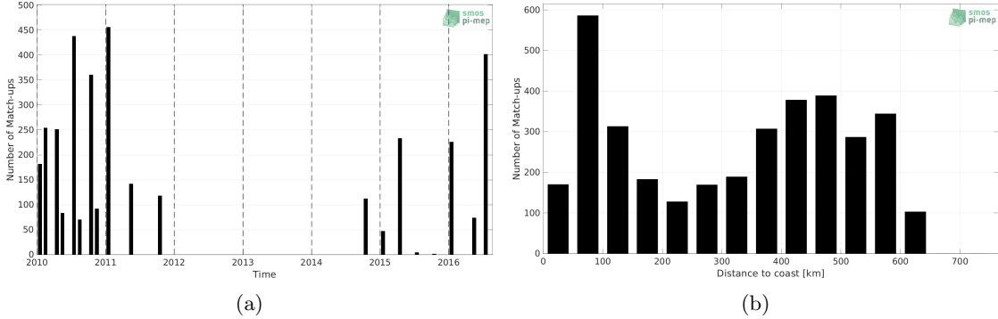
Figure 1: Number of match-ups between TSG (LEGOS-DM) and SMOS SSS L2Q v331 - With FLAG (CMEMS-CATDS-CPDC) SSS as a function of time (a) and as function of the distance to coast (b) over the Ganga and Brahmaputra river plumes Pi-MEP region and for the full satellite product period.
