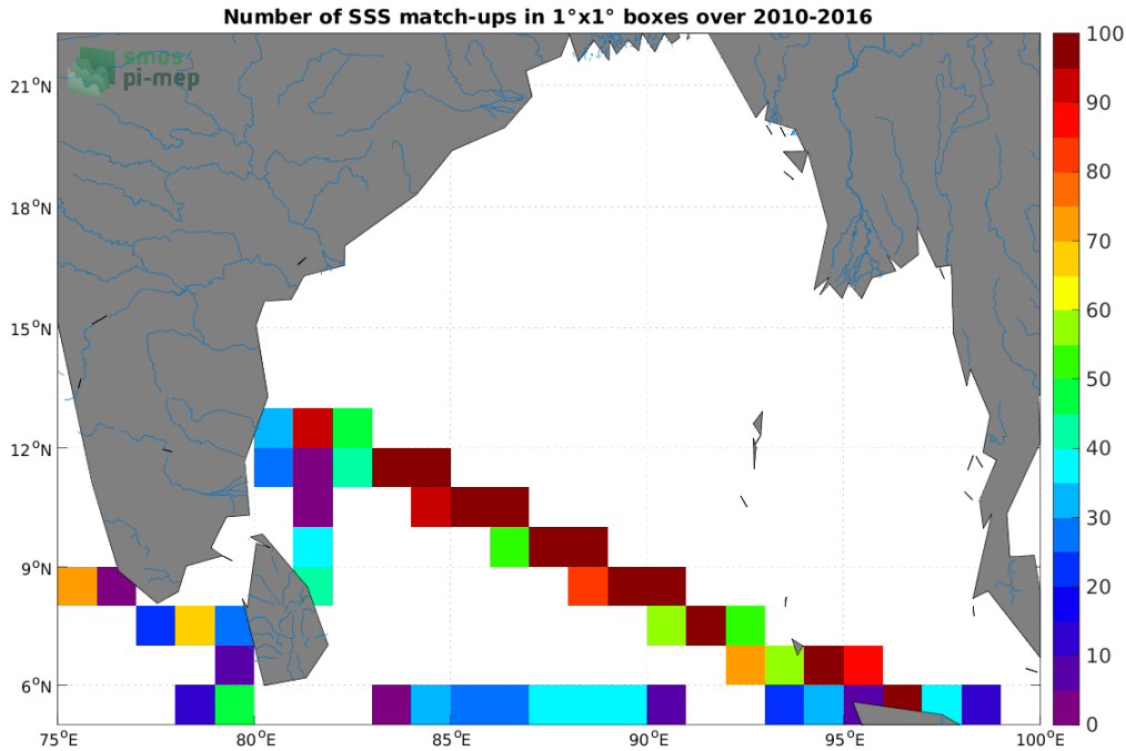
Figure 4: Number of SSS match-ups between TSG (LEGOS-DM) SSS and the SMOS SSS L2Q v331 - With FLAG (CMEMS-CATDS-CPDC) SSS product for the Ganga and Brahmaputra river plumes Pi-MEP region over 1^\circ \times 1^\circ boxes and for the full satellite product period.
