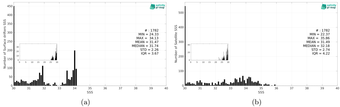
Figure 3: Histograms of SSS from Surface drifters (a) and SMOS SSS L2Q v331 - With FLAG (CMEMS-CATDS-CPDC) (b) considering all match-up pairs per bins of 0.1 over the Ganga and Brahmaputra river plumes Pi-MEP region and for the full satellite product period.
