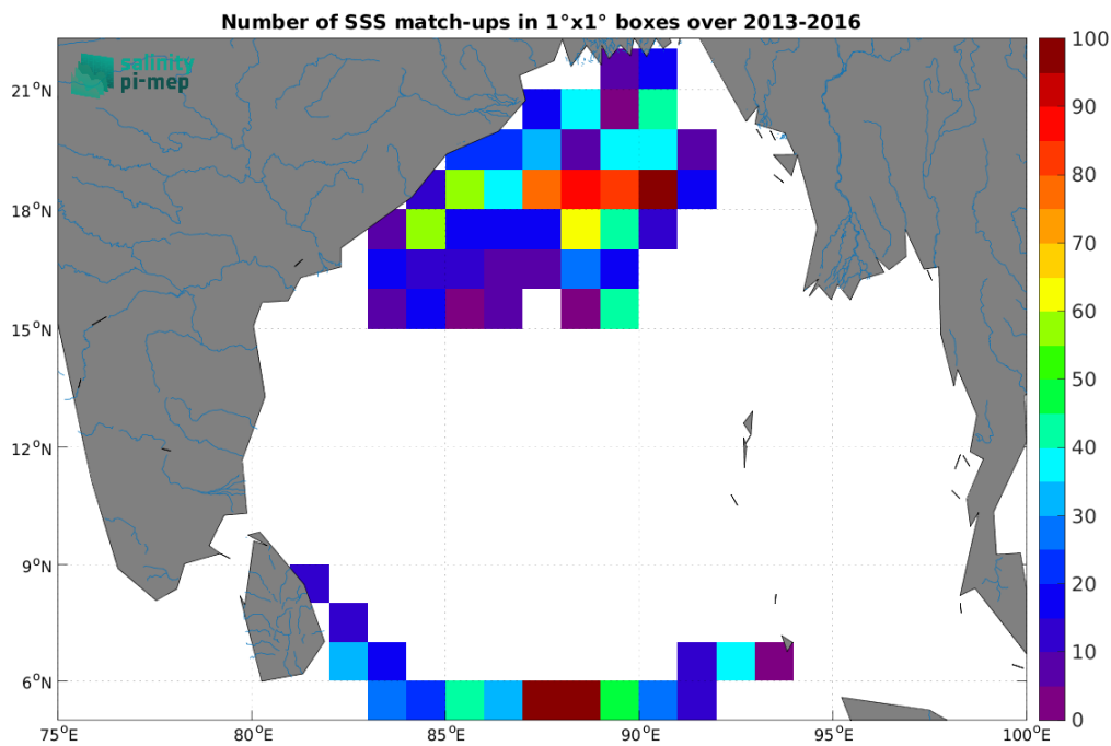
Figure 4: Number of SSS match-ups between Surface drifters SSS and the SMOS SSS L2Q v331 - With FLAG (CMEMS-CATDS-CPDC) SSS product for the Ganga and Brahmaputra river plumes Pi-MEP region over 1^\circ \times 1^\circ boxes and for the full satellite product period.
