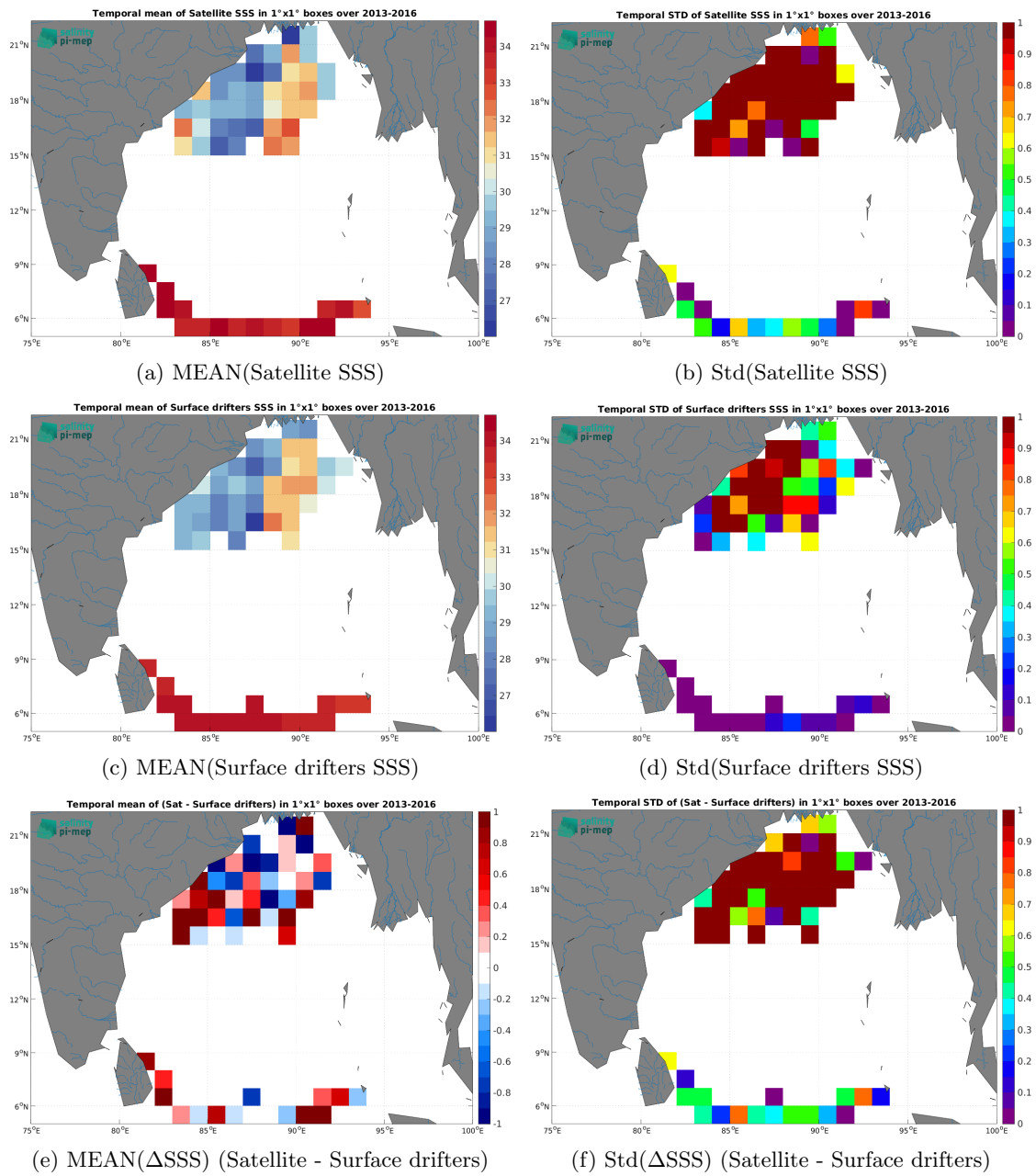
Figure 5: Temporal mean (left) and Std (right) of SSS from SMOS SSS L2Q v331 - With FLAG (CMEMS-CATDS-CPDC) (top), Surface drifters (middle), and of \Delta SSS (Satellite - Surface drifters). Only match-up pairs are used to generate these maps.
