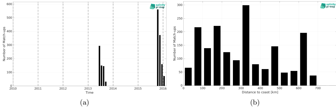
Figure 1: Number of match-ups between Surface drifters and SMOS SSS L2Q v331 - With FLAG (CMEMS-CATDS-CPDC) SSS as a function of time (a) and as function of the distance to coast (b) over the Ganga and Brahmaputra river plumes Pi-MEP region and for the full satellite product period.
