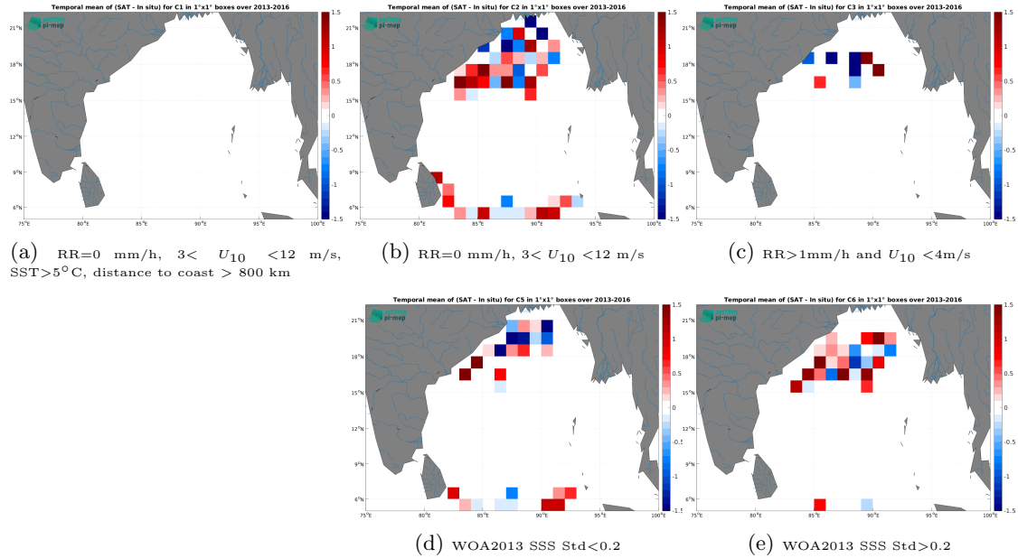
Figure 11: Temporal mean gridded over spatial boxes of size 1^{\circ}\times 1^{\circ} of \Delta\text{SSS} (SMOS SSS L2Q v331 - With FLAG (CMEMS-CATDS-CPDC) - Surface drifters) for 5 different subdatasets corresponding to:RR=0 mm/h, 3 < U_{10} < 12 m/s, SST >5^{\circ}\text{C} , distance to coast > 800 km (a), RR=0 mm/h, 3 < U_{10} < 12 m/s (b), RR >1 mm/h and U_{10} < 4 m/s (c), WOA2013 SSS Std <0.2 (d), WOA2013 SSS Std >0.2 (e).
