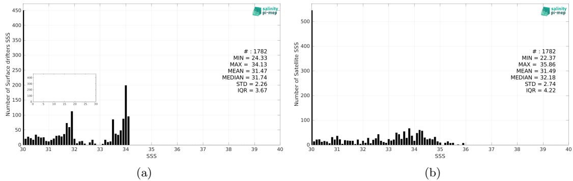
Figure 2: Histograms of SSS from Surface drifters (a) and SMOS SSS L2Q v331 - With FLAG (CMEMS-CATDS-CPDC) (b) considering all match-up pairs per bins of 0.1 over the Ganga and Brahmaputra river plumes Pi-MEP region and for the full satellite product period.
