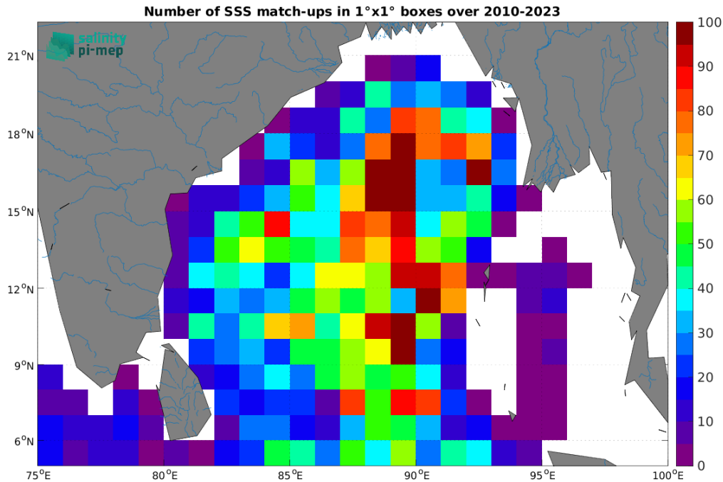
Figure 5: Number of SSS match-ups between Argo SSS and the SMOS SSS L2Q v331 - With FLAG (CMEMS-CATDS-CPDC) SSS product for the Ganga and Brahmaputra river plumes Pi-MEP region over 1^\circ \times 1^\circ boxes and for the full satellite product period.
