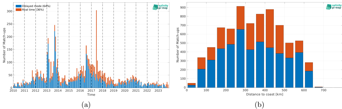
Figure 2: Number of match-ups between Argo and SMOS SSS L2Q v331 - With FLAG (CMEMS-CATDS-CPDC) SSS as a function of time (a) and as function of the distance to coast (b) over the Ganga and Brahmaputra river plumes Pi-MEP region and for the full satellite product period.
