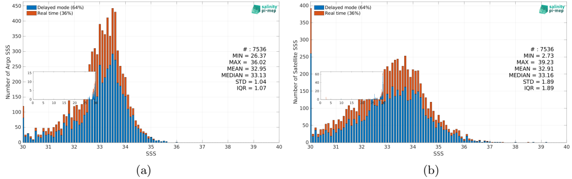
Figure 3: Histograms of SSS from Argo (a) and SMOS SSS L2Q v331 - With FLAG (CMEMS-CATDS-CPDC) (b) considering all match-up pairs per bins of 0.1 over the Ganga and Brahmaputra river plumes Pi-MEP region and for the full satellite product period.
