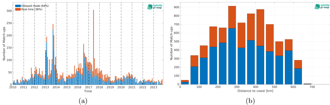
Figure 1: Number of match-ups between Argo and SMOS SSS L2Q v331 - With FLAG (CMEMS-CATDS-CPDC) SSS as a function of time (a) and as function of the distance to coast (b) over the Ganga and Brahmaputra river plumes Pi-MEP region and for the full satellite product period.
