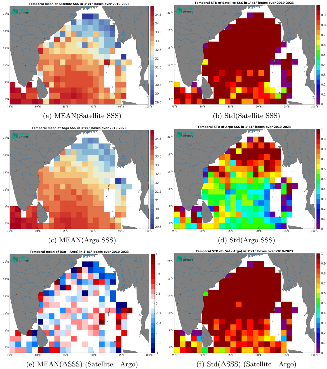
Figure 6: Temporal mean (left) and Std (right) of SSS from SMOS SSS L2Q v331 - With FLAG (CMEMS-CATDS-CPDC) (top), Argo (middle), and of \Delta SSS (Satellite - Argo). Only match-up pairs are used to generate these maps.
