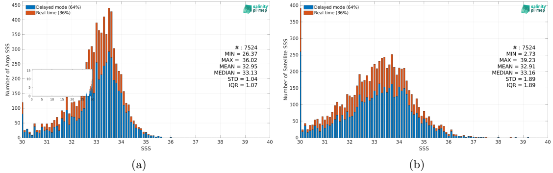
Figure 2: Histograms of SSS from Argo (a) and SMOS SSS L2Q v331 - With FLAG (CMEMS-CATDS-CPDC) (b) considering all match-up pairs per bins of 0.1 over the Ganga and Brahmaputra river plumes Pi-MEP region and for the full satellite product period.
