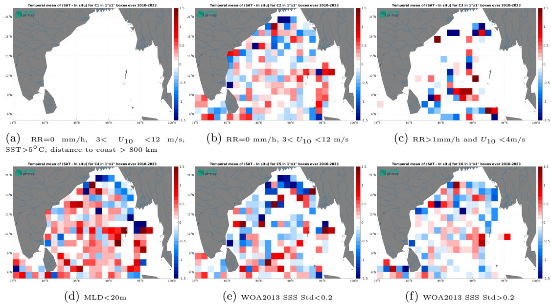
Figure 12: Temporal mean gridded over spatial boxes of size 1^\circ \times 1^\circ of \Delta SSS (SMOS SSS L2Q v331 - With FLAG (CMEMS-CATDS-CPDC) - Argo) for 6 different subdatasets corresponding to:RR=0 mm/h, 3 < U_{10} < 12 m/s, SST >5^\circ C, distance to coast > 800 km (a), RR=0 mm/h, 3 < U_{10} < 12 m/s (b), RR >1 mm/h and U_{10} < 4 m/s (c),MLD <20 m (d),WOA2013 SSS Std <0.2 (e),WOA2013 SSS Std >0.2 (f).
