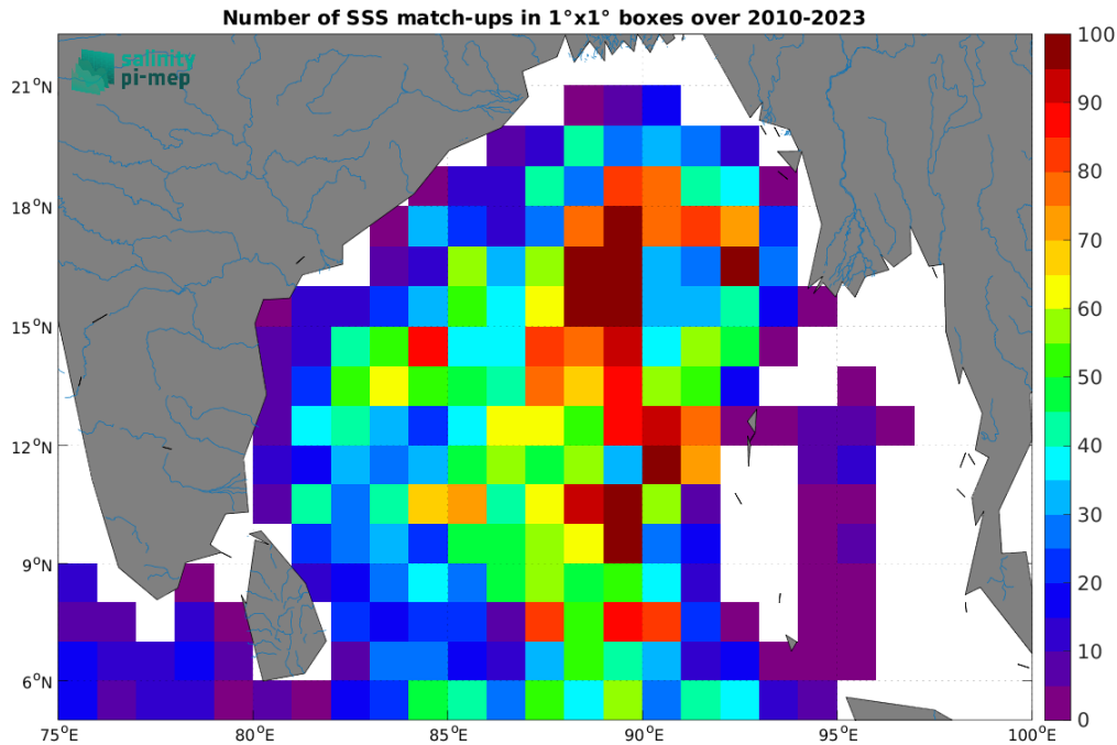
Figure 4: Number of SSS match-ups between Argo SSS and the SMOS SSS L2Q v331 - With FLAG (CMEMS-CATDS-CPDC) SSS product for the Ganga and Brahmaputra river plumes Pi-MEP region over 1^{\circ} \times 1^{\circ} boxes and for the full satellite product period.
