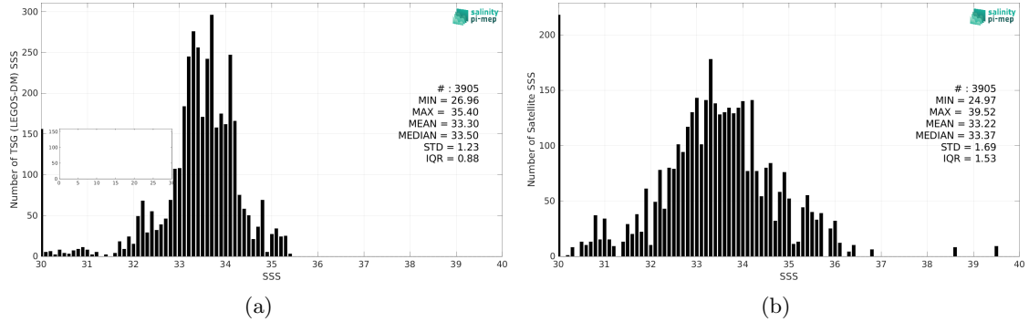
Figure 2: Histograms of SSS from TSG (LEGOS-DM) (a) and SMOS SSS L2Q v331 - No FLAG (CMEMS-CATDS-CPDC) (b) considering all match-up pairs per bins of 0.1 over the Ganga and Brahmaputra river plumes Pi-MEP region and for the full satellite product period.
