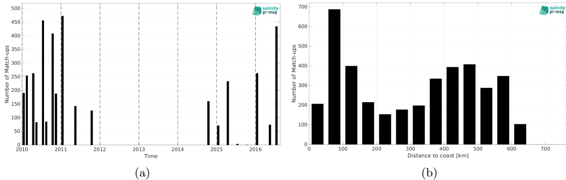
Figure 1: Number of match-ups between TSG (LEGOS-DM) and SMOS SSS L2Q v331 - No FLAG (CMEMS-CATDS-CPDC) SSS as a function of time (a) and as function of the distance to coast (b) over the Ganga and Brahmaputra river plumes Pi-MEP region and for the full satellite product period.
