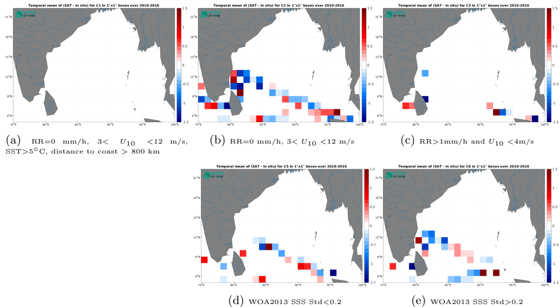
Figure 12: Temporal mean gridded over spatial boxes of size 1^{\circ}\times 1^{\circ} of \Delta\text{SSS} (SMOS SSS L2Q v331 - No FLAG (CMEMS-CATDS-CPDC) - TSG (LEGOS-DM)) for 5 different subdatasets corresponding to:RR=0 mm/h, 3 < U_{10} < 12 m/s, SST > 5^{\circ}\text{C} , distance to coast > 800 km (a), RR=0 mm/h, 3 < U_{10} < 12 m/s (b), RR > 1 mm/h and U_{10} < 4 m/s (c), WOA2013 SSS Std < 0.2 (d), WOA2013 SSS Std > 0.2 (e).
