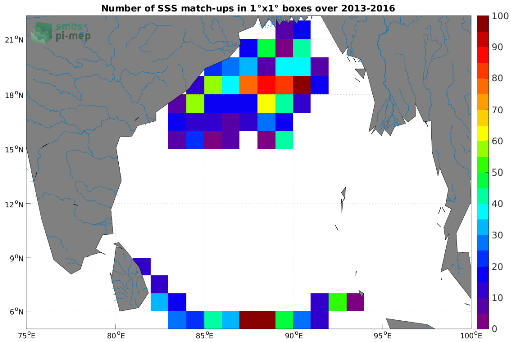
Figure 3: Number of SSS match-ups between Surface drifters SSS and the SMOS SSS L2Q v331 - No FLAG (CMEMS-CATDS-CPDC) SSS product for the Ganga and Brahmaputra river plumes Pi-MEP region over 1^\circ \times 1^\circ boxes and for the full satellite product period.
