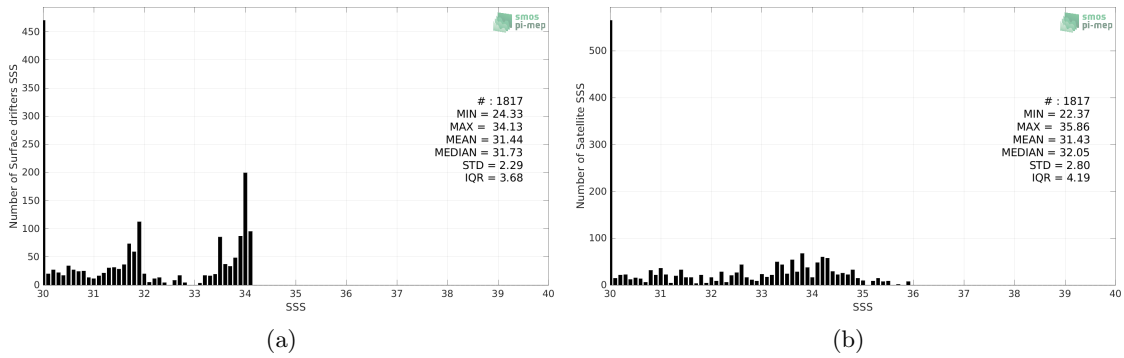
Figure 2: Histograms of SSS from Surface drifters (a) and SMOS SSS L2Q v331 - No FLAG (CMEMS-CATDS-CPDC) (b) considering all match-up pairs per bins of 0.1 over the Ganga and Brahmaputra river plumes Pi-MEP region and for the full satellite product period.
