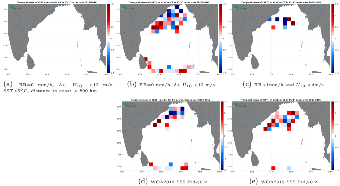
Figure 11: Temporal mean gridded over spatial boxes of size 1^{\circ}\times 1^{\circ} of \Delta\text{SSS} (SMOS SSS L2Q v331 - No FLAG (CMEMS-CATDS-CPDC) - Surface drifters) for 5 different subdatasets corresponding to:RR=0 mm/h, 3 < U_{10} < 12 m/s, SST > 5^{\circ}\text{C} , distance to coast > 800 km (a), RR=0 mm/h, 3 < U_{10} < 12 m/s (b), RR > 1 mm/h and U_{10} < 4 m/s (c), WOA2013 SSS Std < 0.2 (d), WOA2013 SSS Std > 0.2 (e).
