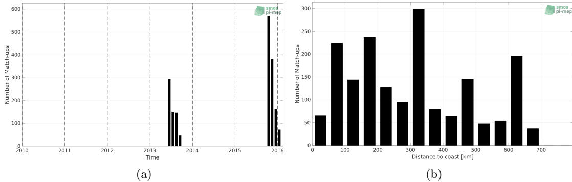
Figure 1: Number of match-ups between Surface drifters and SMOS SSS L2Q v331 - No FLAG (CMEMS-CATDS-CPDC) SSS as a function of time (a) and as function of the distance to coast (b) over the Ganga and Brahmaputra river plumes Pi-MEP region and for the full satellite product period.
