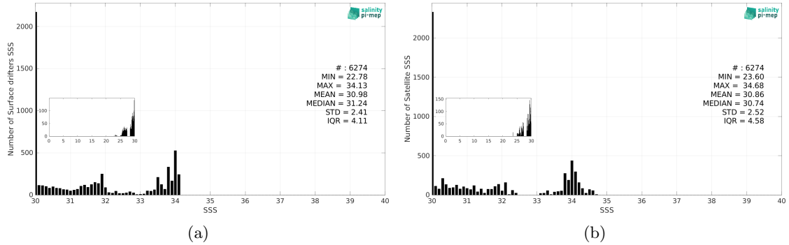
Figure 3: Histograms of SSS from Surface drifters (a) and SMOS SSS L3 v9 - 9 Days (CATDS-CEC-LOCEAN) (b) considering all match-up pairs per bins of 0.1 over the Ganga and Brahmaputra river plumes Pi-MEP region and for the full satellite product period.
