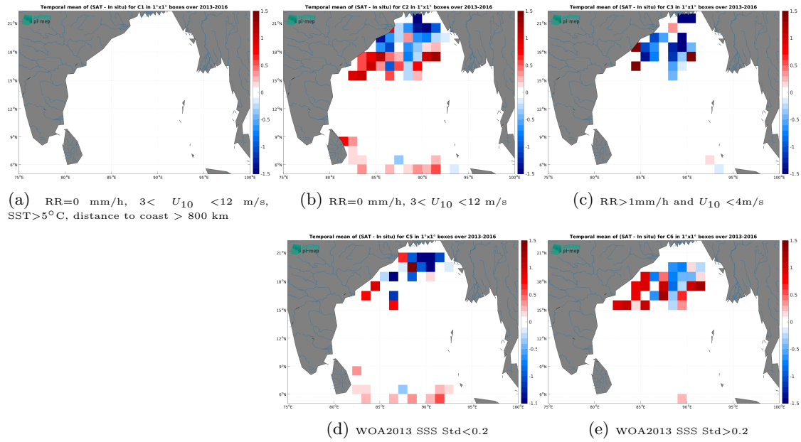
Figure 13: Temporal mean gridded over spatial boxes of size 1^\circ \times 1^\circ of \Delta SSS (SMOS SSS L3 v9 - 9 Days (CATDS-CEC-LOCEAN) - Surface drifters) for 5 different subdatasets corresponding to:RR=0 mm/h, 3 < U_{10} < 12 m/s, SST >5^\circ C, distance to coast > 800 km (a), RR=0 mm/h, 3 < U_{10} < 12 m/s (b), RR >1 mm/h and U_{10} < 4 m/s (c), WOA2013 SSS Std <0.2 (d), WOA2013 SSS Std >0.2 (e).
