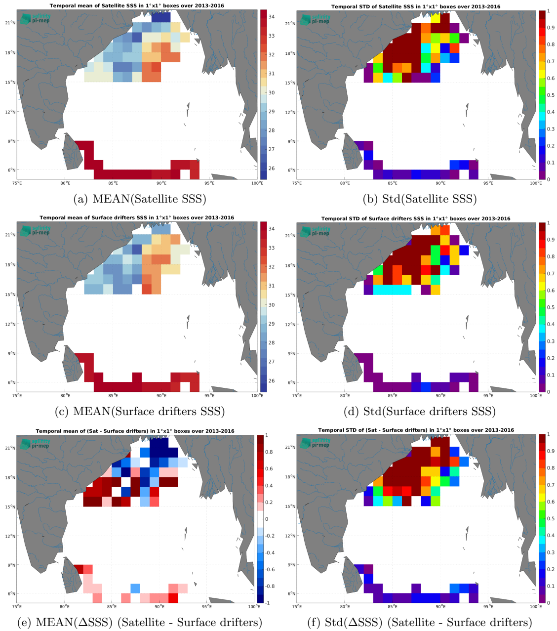
Figure 6: Temporal mean (left) and Std (right) of SSS from SMOS SSS L3 v9 - 9 Days (CATDS-CEC-LOCEAN) (top), Surface drifters (middle), and of \Delta SSS (Satellite - Surface drifters). Only match-up pairs are used to generate these maps.
