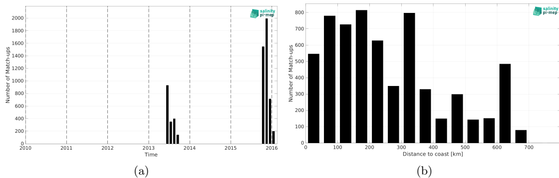
Figure 2: Number of match-ups between Surface drifters and SMOS SSS L3 v9 - 9 Days (CATDS-CEC-LOCEAN) SSS as a function of time (a) and as function of the distance to coast (b) over the Ganga and Brahmaputra river plumes Pi-MEP region and for the full satellite product period.
