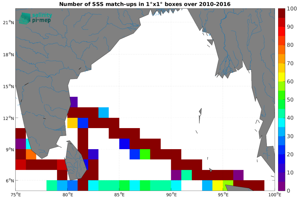
Figure 4: Number of SSS match-ups between TSG (LEGOS-DM) SSS and the SMOS SSS L3 v8 - 9 Days (CATDS-CEC-LOCEAN) SSS product for the Ganga and Brahmaputra river plumes Pi-MEP region over 1^\circ \times 1^\circ boxes and for the full satellite product period.
