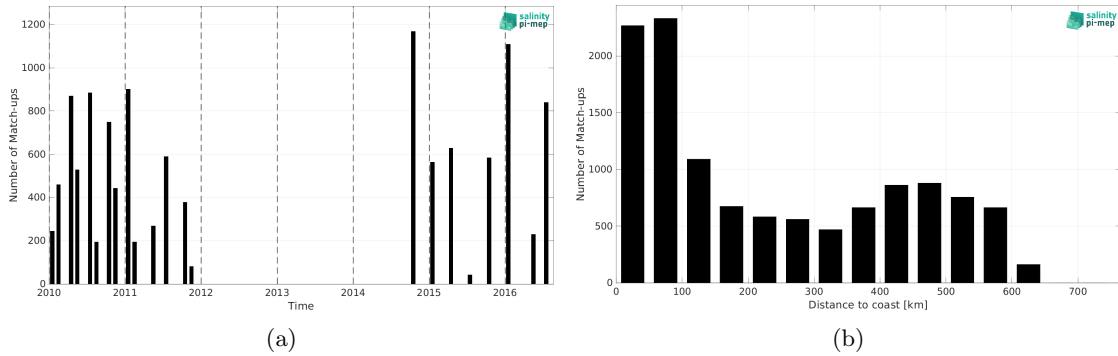
Figure 1: Number of match-ups between TSG (LEGOS-DM) and SMOS SSS L3 v8 - 9 Days (CATDS-CEC-LOCEAN) SSS as a function of time (a) and as function of the distance to coast (b) over the Ganga and Brahmaputra river plumes Pi-MEP region and for the full satellite product period.
