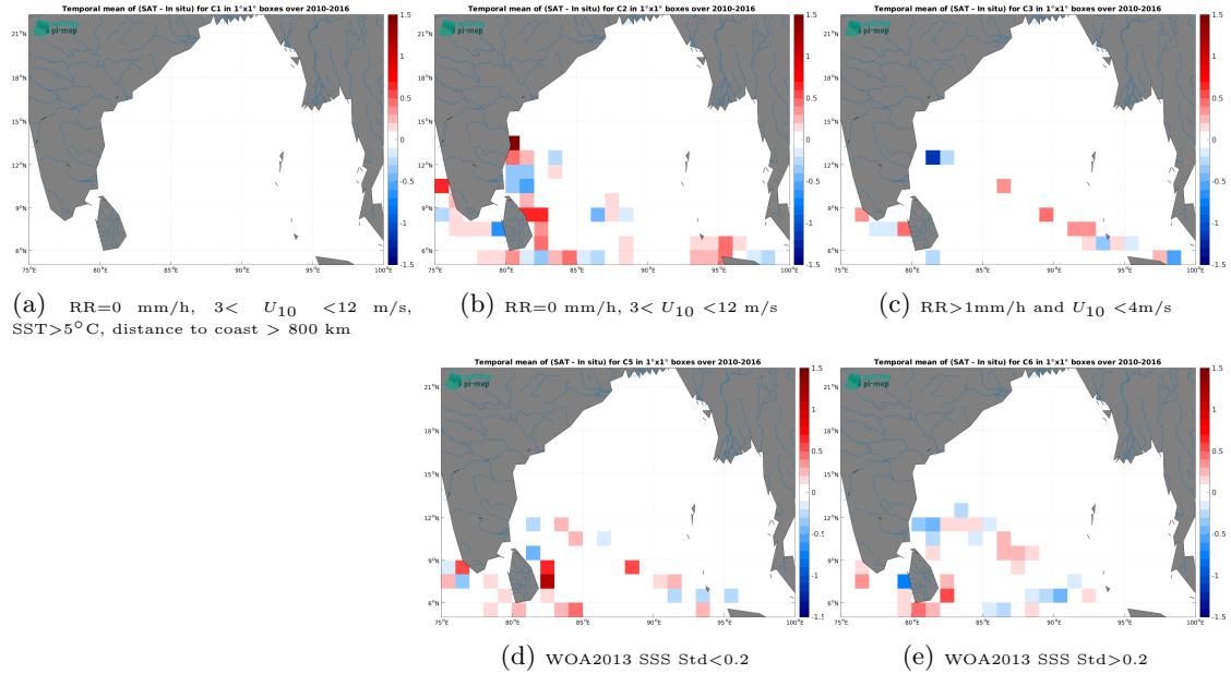
Figure 12: Temporal mean gridded over spatial boxes of size 1^{\circ}\times 1^{\circ} of \Delta\text{SSS} (SMOS SSS L3 v8 - 9 Days (CATDS-CEC-LOCEAN) - TSG (LEGOS-DM)) for 5 different subdatasets corresponding to:RR=0 mm/h, 3 < U_{10} < 12 m/s, SST >5^{\circ}\text{C} , distance to coast > 800 km (a), RR=0 mm/h, 3 < U_{10} < 12 m/s (b), RR >1 mm/h and U_{10} < 4 m/s (c), WOA2013 SSS Std <0.2 (d), WOA2013 SSS Std >0.2 (e).
