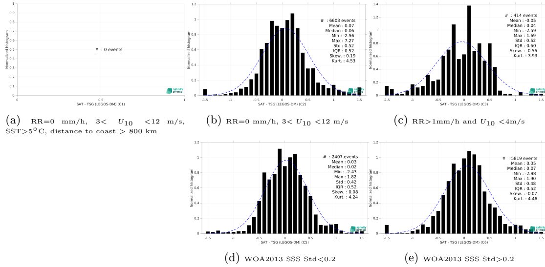
Figure 13: Normalized histogram of \Delta SSS (SMOS SSS L3 v8 - 9 Days (CATDS-CEC-LOCEAN) - TSG (LEGOS-DM)) for 5 different subdatasets corresponding to: RR=0 mm/h, 3 < U_{10} < 12 m/s, SST>5°C, distance to coast > 800 km (a), RR=0 mm/h, 3 < U_{10} < 12 m/s (b), RR>1mm/h and U_{10} < 4 m/s (c), WOA2013 SSS Std<0.2 (d), WOA2013 SSS Std>0.2 (e).
