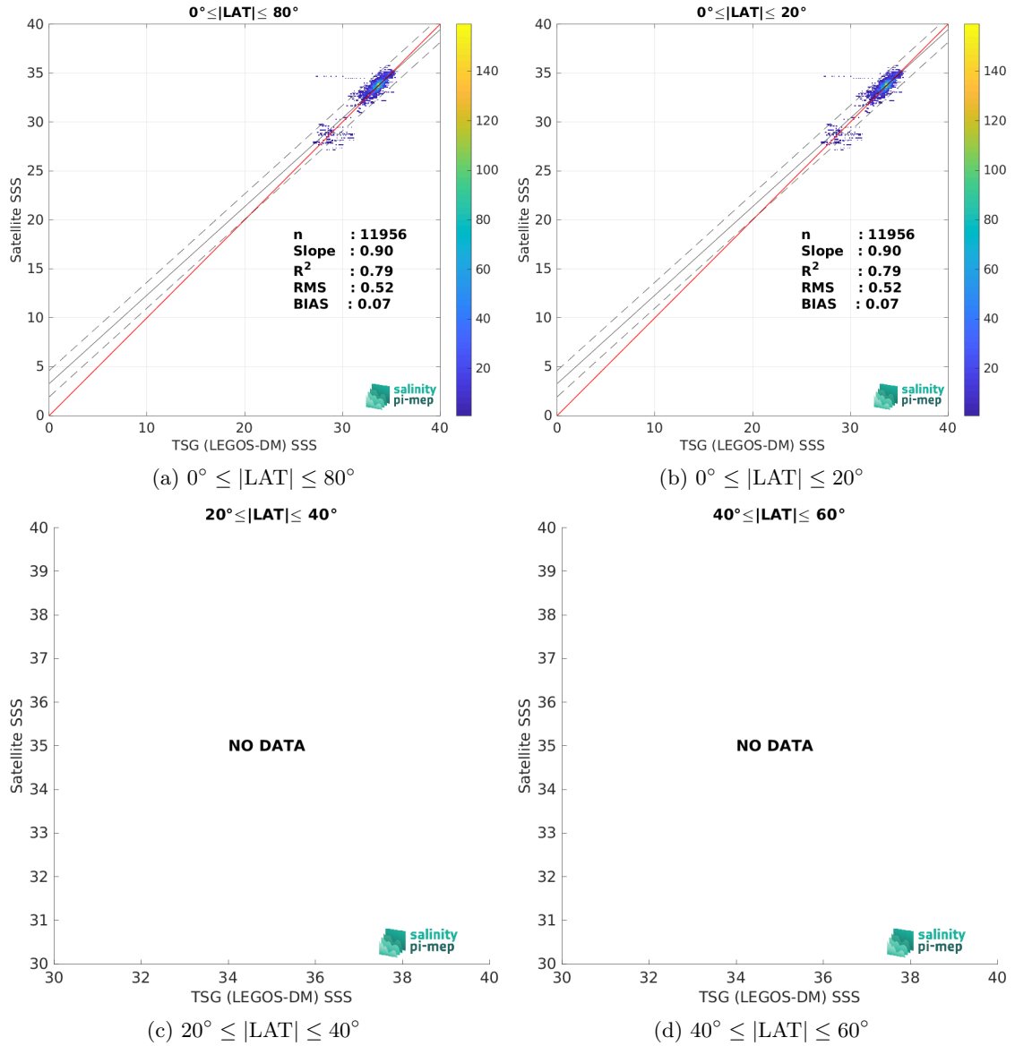
Figure 9: Contour maps of the concentration of SMOS SSS L3 v8 - 9 Days (CATDS-CEC-LOCEAN) SSS (y-axis) versus TSG (LEGOS-DM) SSS (x-axis) at match-up pairs for different latitude bands. For each plot, the red line shows x=y . The black thin and dashed lines indicate a linear fit through the data cloud and the \pm 95\% confidence levels, respectively. The number match-up pairs n , the slope and R^2 coefficient of the linear fit, the root mean square (RMS) and the mean bias between satellite and in situ data are indicated for each latitude band in each plots.
