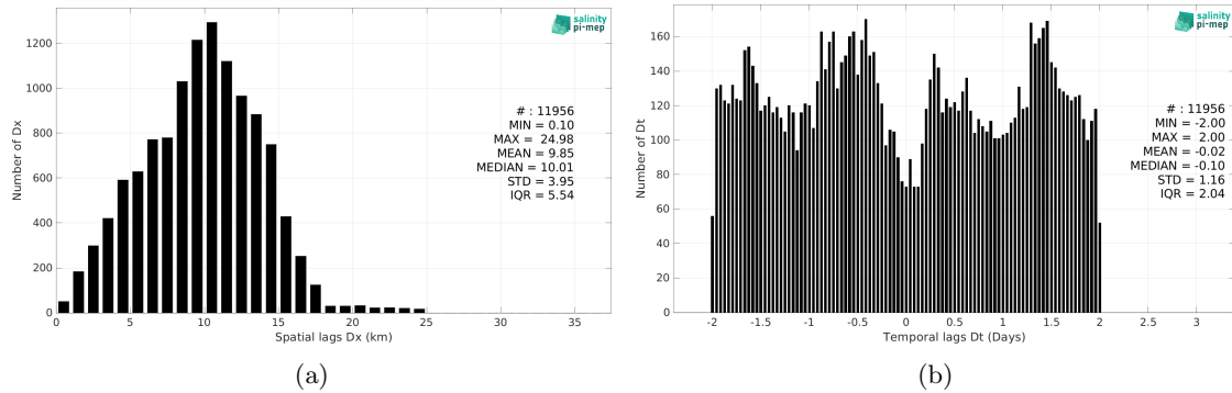
Figure 5: Histograms of the spatial (a) and temporal (b) lags between the location/time of the TSG (LEGOS-DM) measurement and the date of the corresponding SMOS SSS L3 v8 - 9 Days (CATDS-CEC-LOCEAN) SSS pixel.
