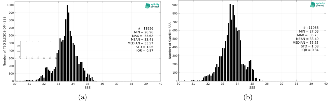
Figure 2: Histograms of SSS from TSG (LEGOS-DM) (a) and SMOS SSS L3 v8 - 9 Days (CATDS-CEC-LOCEAN) (b) considering all match-up pairs per bins of 0.1 over the Ganga and Brahmaputra river plumes Pi-MEP region and for the full satellite product period.
