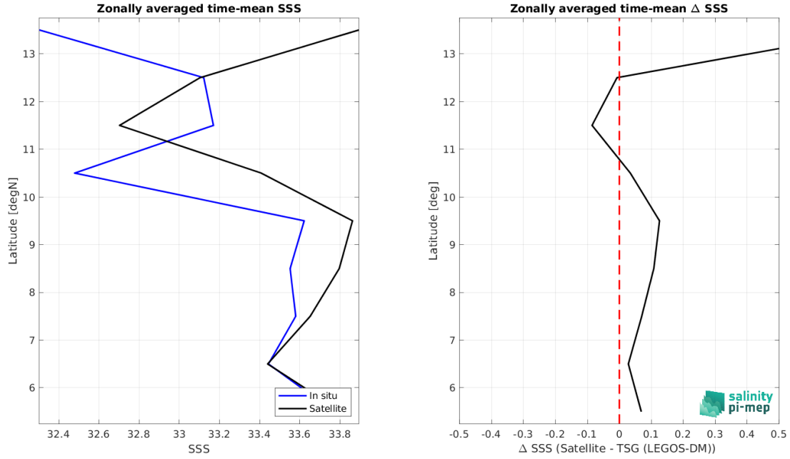
Figure 8: Left panel: Zonal mean SSS from SMOS SSS L3 v8 - 9 Days (CATDS-CEC-LOCEAN) satellite product (black) and from TSG (LEGOS-DM) (blue). Right panel: Zonal mean of \Delta SSS (Satellite - TSG (LEGOS-DM)) for all the collected Pi-MEP match-up pairs estimated over the full satellite product period.
