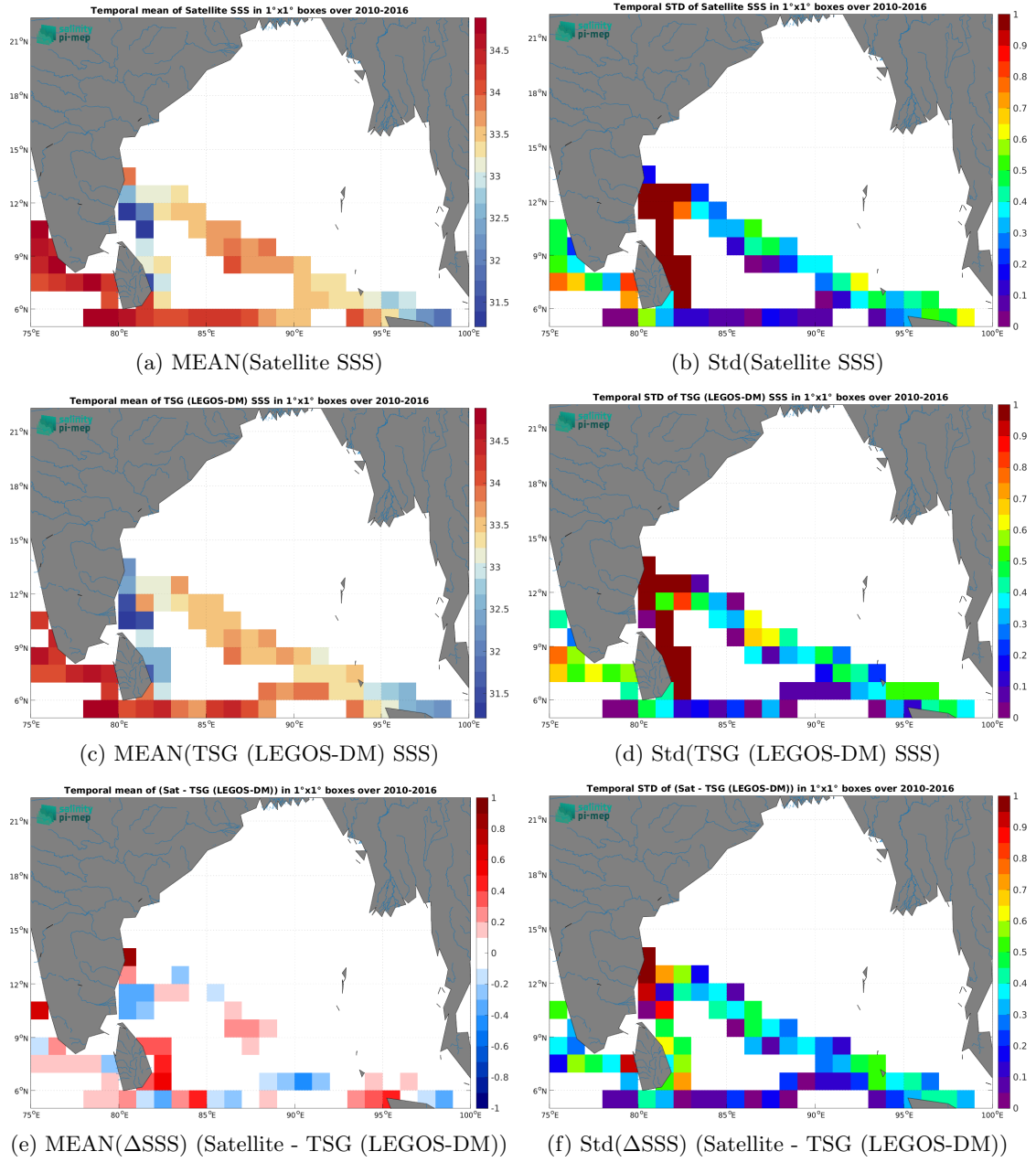
Figure 6: Temporal mean (left) and Std (right) of SSS from SMOS SSS L3 v8 - 9 Days (CATDS-CEC-LOCEAN) (top), TSG (LEGOS-DM) (middle), and of \Delta SSS (Satellite - TSG (LEGOS-DM)). Only match-up pairs are used to generate these maps.
