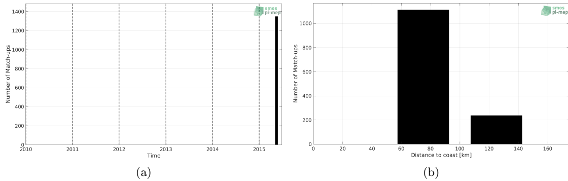
Figure 1: Number of match-ups between TSG (SAMOS) and SMOS SSS L3 v5 - 18 Days (CATDS-CECOS-LOCEAN) SSS as a function of time (a) and as function of the distance to coast (b) over the Ganga and Brahmaputra river plumes Pi-MEP region and for the full satellite product period.
