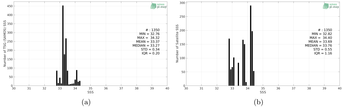
Figure 2: Histograms of SSS from TSG (SAMOS) (a) and SMOS SSS L3 v5 - 18 Days (CATDS-CECOS-LOCEAN) (b) considering all match-up pairs per bins of 0.1 over the Ganga and Brahmaputra river plumes Pi-MEP region and for the full satellite product period.
