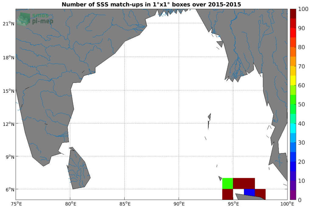
Figure 4: Number of SSS match-ups between TSG (SAMOS) SSS and the SMOS SSS L3 v5 - 18 Days (CATDS-CECOS-LOCEAN) SSS product for the Ganga and Brahmaputra river plumes Pi-MEP region over 1^{\circ} \times 1^{\circ} boxes and for the full satellite product period.
