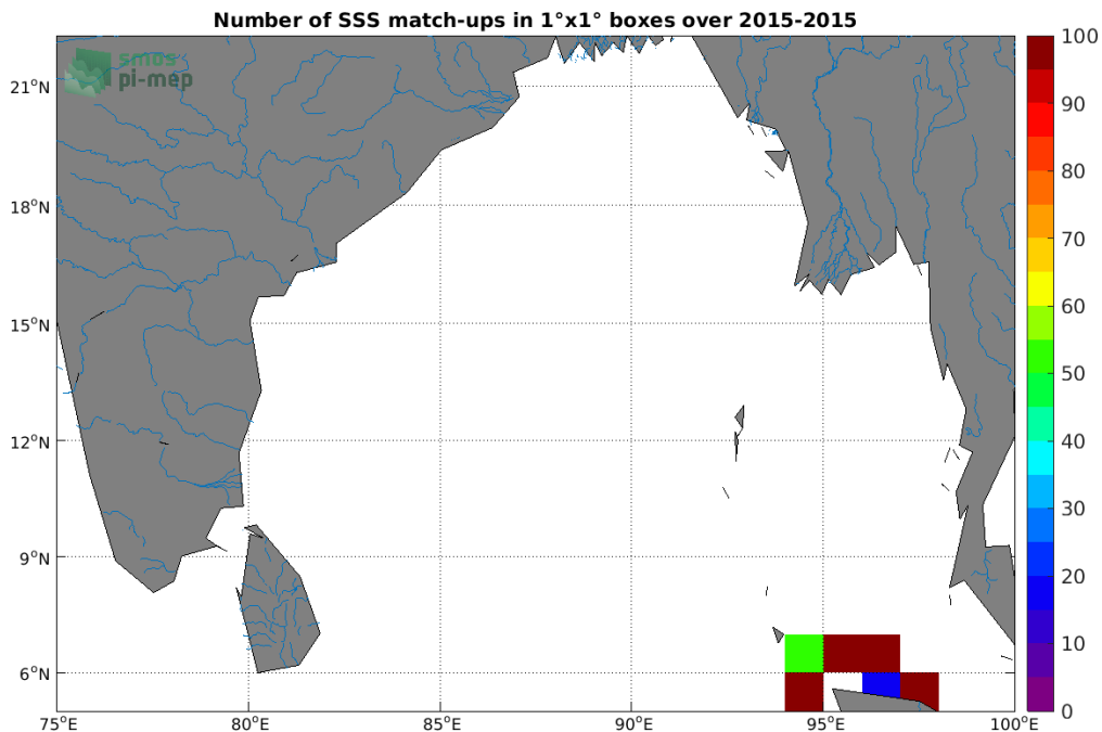
Figure 4: Number of SSS match-ups between TSG (SAMOS) SSS and the SMOS SSS L3 v5 - 18 Days (CATDS-CECOS-LOCEAN) SSS product for the Ganga and Brahmaputra river plumes Pi-MEP region over 1^\circ \times 1^\circ boxes and for the full satellite product period.
