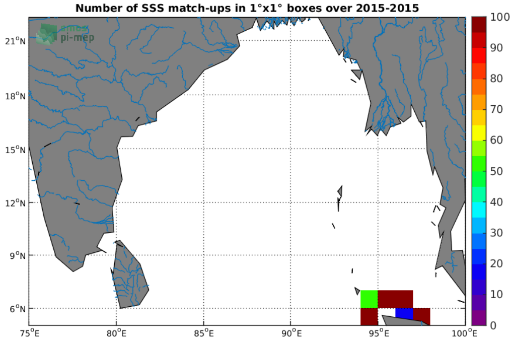
Figure 4: Number of SSS match-ups between TSG-SAMOS SSS and the SMOS-L3-CATDS-CECOS-LOCEAN-V4-9DAYS-25KM SSS product for the Ganga and Brahmaputra river plumes Pi-MEP region over 1°x1° boxes and for the full satellite product period.
