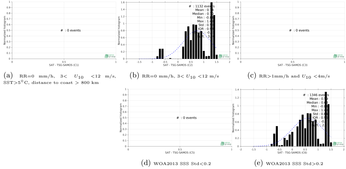
Figure 13: Normalized histogram of \Delta SSS (SMOS-L3-CATDS-CECOS-LOCEAN-V4-9DAYS-25KM - TSG-SAMOS) for 5 different subdatasets corresponding to: RR=0 mm/h, 3 < U_{10} < 12 m/s, SST>5°C, distance to coast > 800 km (a), RR=0 mm/h, 3 < U_{10} < 12 m/s (b), RR>1mm/h and U_{10} < 4 m/s (c), WOA2013 SSS Std<0.2 (d), WOA2013 SSS Std>0.2 (e).
