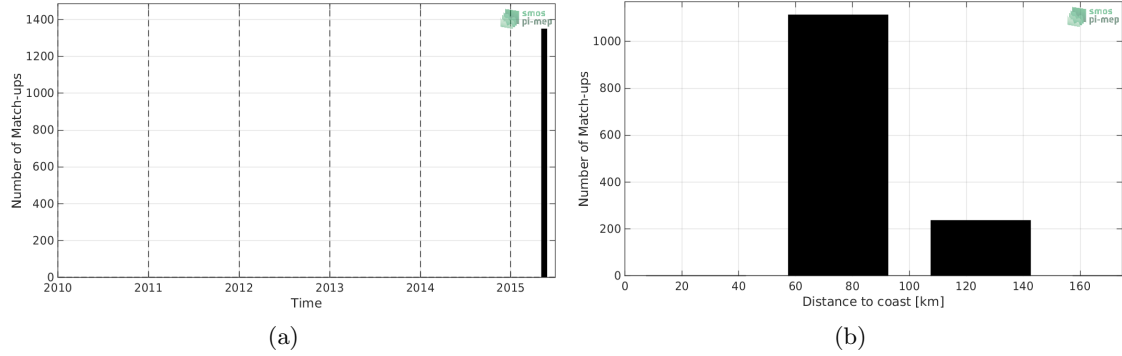
Figure 1: Number of match-ups between TSG-SAMOS and SMOS-L3-CATDS-CECOS-LOCEAN-V4-9DAYS-25KM SSS as a function of time (a) and as function of the distance to coast (b) over the Ganga and Brahmaputra river plumes Pi-MEP region and for the full satellite product period.
