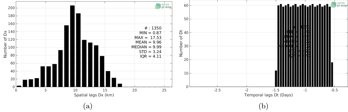
Figure 5: Histograms of the spatial (a) and temporal (b) lags between the time of the TSG-SAMOS measurements and the date of the corresponding SMOS-L3-CATDS-CECOS-LOCEAN-V4-9DAYS-25KM SSS product.
