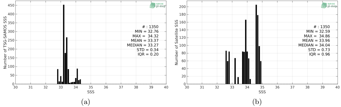
Figure 2: Histograms of SSS from TSG-SAMOS (a) and SMOS-L3-CATDS-CECOS-LOCEAN-V4-9DAYS-25KM (b) considering all match-up pairs per bins of 0.1 over the Ganga and Brahmaputra river plumes Pi-MEP region and for the full satellite product period.
