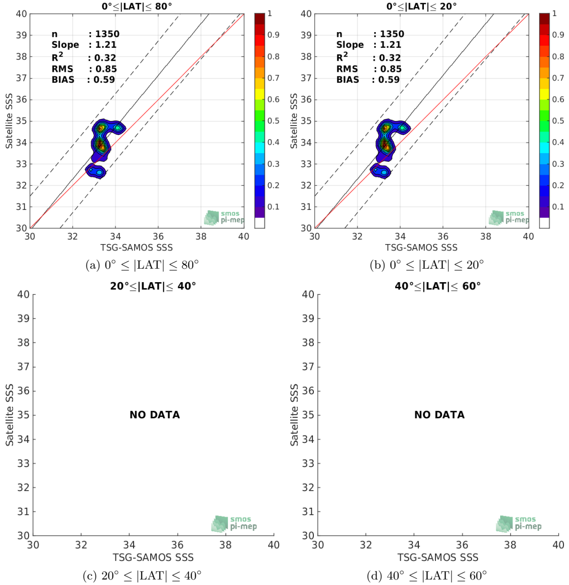
Figure 9: Contour maps of the concentration of SMOS-L3-CATDS-CECOS-LOCEAN-V4-9DAYS-25KM SSS (y-axis) versus TSG-SAMOS SSS (x-axis) at match-up pairs for different latitude bands. For each plot, the red line shows x=y . The black thin and dashed lines indicate a linear fit through the data cloud and the \pm 95\% confidence levels, respectively. The number match-up pairs n , the slope and R^2 coefficient of the linear fit, the root mean square (RMS) and the mean bias between satellite and in situ data are indicated for each latitude band in each plots.
