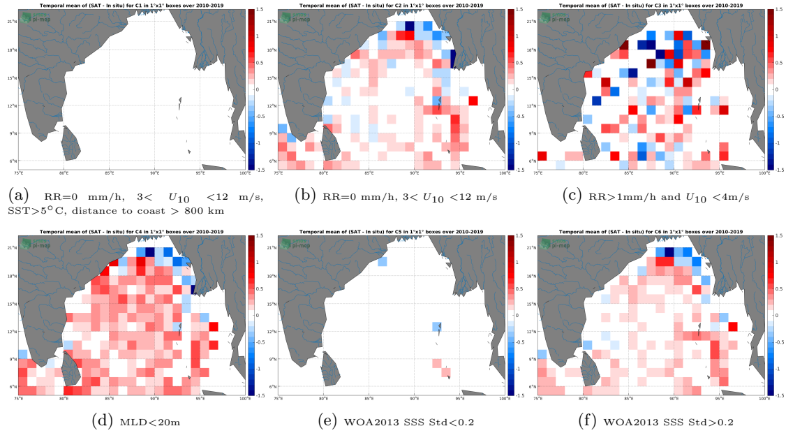
Figure 12: Temporal mean gridded over spatial boxes of size 1^\circ \times 1^\circ of \Delta SSS (SMOS SSS L3 v4 - 9 Days (CATDS-CECOS-LOCEAN) - Argo) for 6 different subdatasets corresponding to: RR=0 mm/h, 3 < U_{10} < 12 m/s, SST > 5^\circ C , distance to coast > 800 km (a), RR=0 mm/h, 3 < U_{10} < 12 m/s (b), RR > 1 mm/h and U_{10} < 4 m/s (c), MLD < 20 m (d), WOA2013 SSS Std < 0.2 (e), WOA2013 SSS Std > 0.2 (f).
