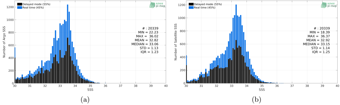
Figure 2: Histograms of SSS from Argo (a) and SMOS SSS L3 v4 - 9 Days (CATDS-CECOS-LOCEAN) (b) considering all match-up pairs per bins of 0.1 over the Ganga and Brahmaputra river plumes Pi-MEP region and for the full satellite product period.
