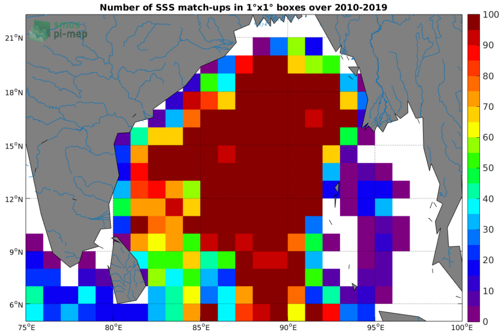
Figure 4: Number of SSS match-ups between Argo SSS and the SMOS SSS L3 v4 - 9 Days (CATDS-CECOS-LOCEAN) SSS product for the Ganga and Brahmaputra river plumes Pi-MEP region over 1°x1° boxes and for the full satellite product period.
