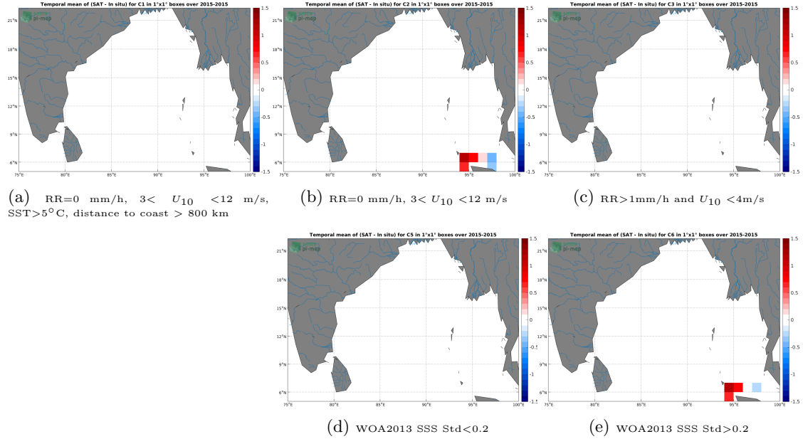
Figure 12: Temporal mean gridded over spatial boxes of size 1^{\circ}\times 1^{\circ} of \Delta\text{SSS} (SMOS SSS L3 v4 - 18 Days (CATDS-CECOS-LOCEAN) - TSG (SAMOS)) for 5 different subdatasets corresponding to: RR=0 mm/h, 3 < U_{10} < 12 m/s, SST > 5^{\circ}\text{C} , distance to coast > 800 km (a), RR=0 mm/h, 3 < U_{10} < 12 m/s (b), RR > 1 mm/h and U_{10} < 4 m/s (c), WOA2013 SSS Std < 0.2 (d), WOA2013 SSS Std > 0.2 (e).
