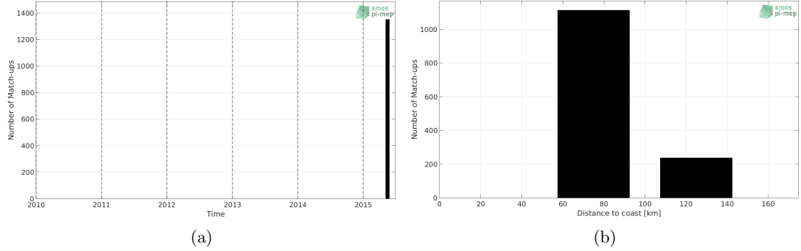
Figure 1: Number of match-ups between TSG (SAMOS) and SMOS SSS L3 v4 - 18 Days (CATDS-CECOS-LOCEAN) SSS as a function of time (a) and as function of the distance to coast (b) over the Ganga and Brahmaputra river plumes Pi-MEP region and for the full satellite product period.
