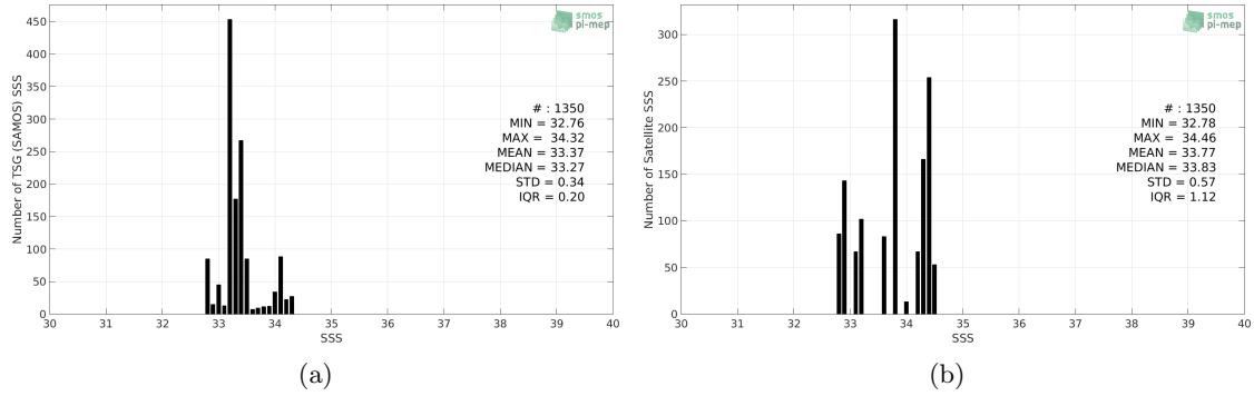
Figure 2: Histograms of SSS from TSG (SAMOS) (a) and SMOS SSS L3 v4 - 18 Days (CATDS-CECOS-LOCEAN) (b) considering all match-up pairs per bins of 0.1 over the Ganga and Brahmaputra river plumes Pi-MEP region and for the full satellite product period.
