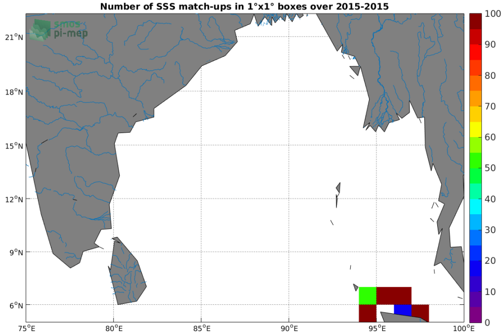
Figure 4: Number of SSS match-ups between TSG (SAMOS) SSS and the SMOS SSS L3 v4 - 18 Days (CATDS-CECOS-LOCEAN) SSS product for the Ganga and Brahmaputra river plumes Pi-MEP region over 1^\circ \times 1^\circ boxes and for the full satellite product period.
