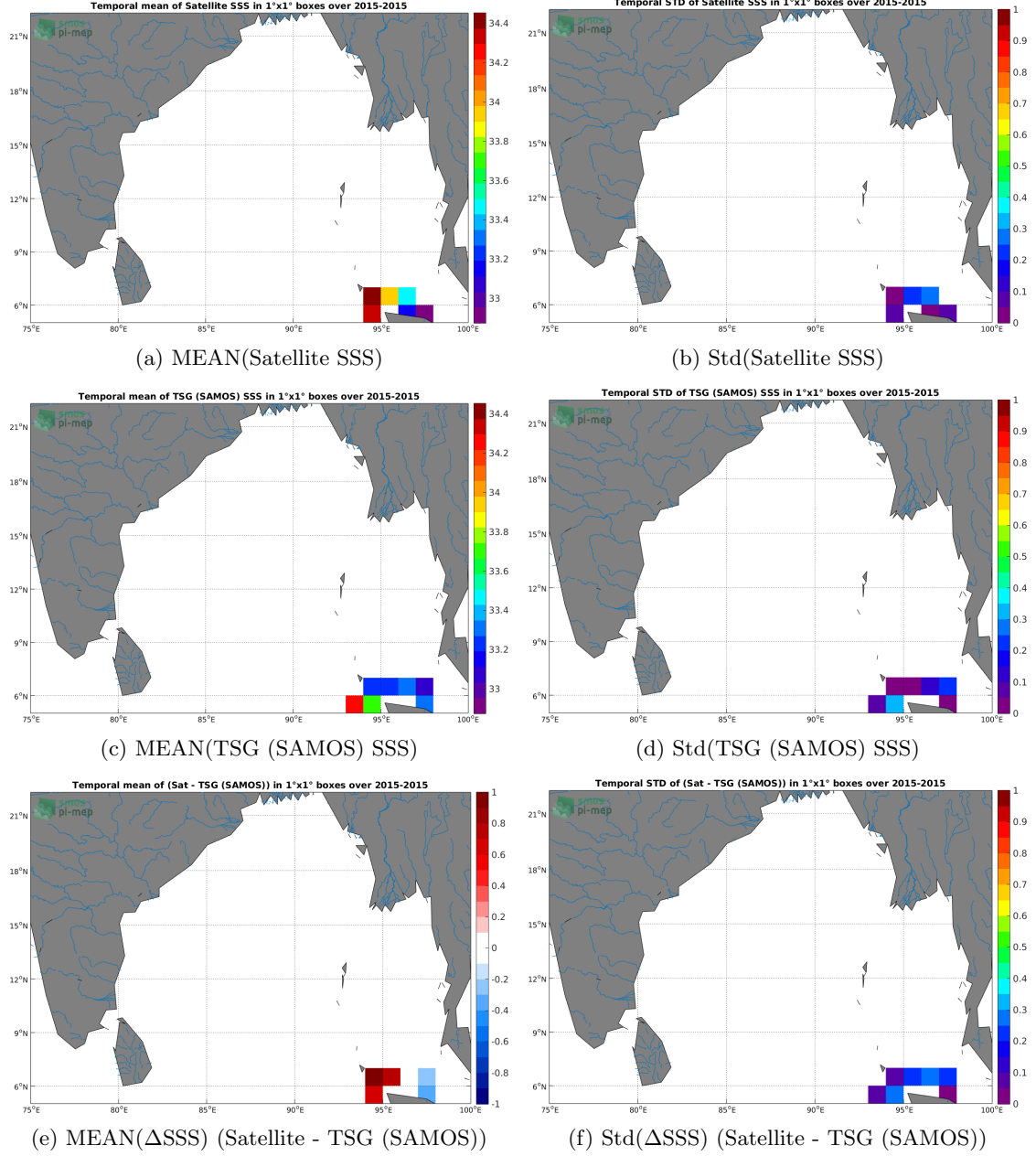
Figure 6: Temporal mean (left) and Std (right) of SSS from SMOS SSS L3 v4 - 18 Days (CATDS-CECOS-LOCEAN) (top), TSG (SAMOS) (middle), and of \Delta SSS (Satellite - TSG (SAMOS)). Only match-up pairs are used to generate these maps.
