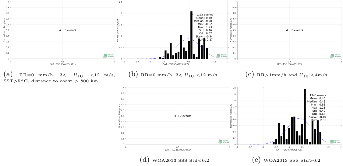
Figure 13: Normalized histogram of \Delta\text{SSS} (SMOS SSS L3 v4 - 18 Days (CATDS-CECOS-LOCEAN) - TSG (SAMOS)) for 5 different subdatasets corresponding to: RR=0 mm/h, 3 < U_{10} < 12 m/s, SST > 5^\circ\text{C} , distance to coast > 800 km (a), RR=0 mm/h, 3 < U_{10} < 12 m/s (b), RR > 1\text{mm/h} and U_{10} < 4\text{m/s} (c), WOA2013 SSS Std < 0.2 (d), WOA2013 SSS Std > 0.2 (e).
