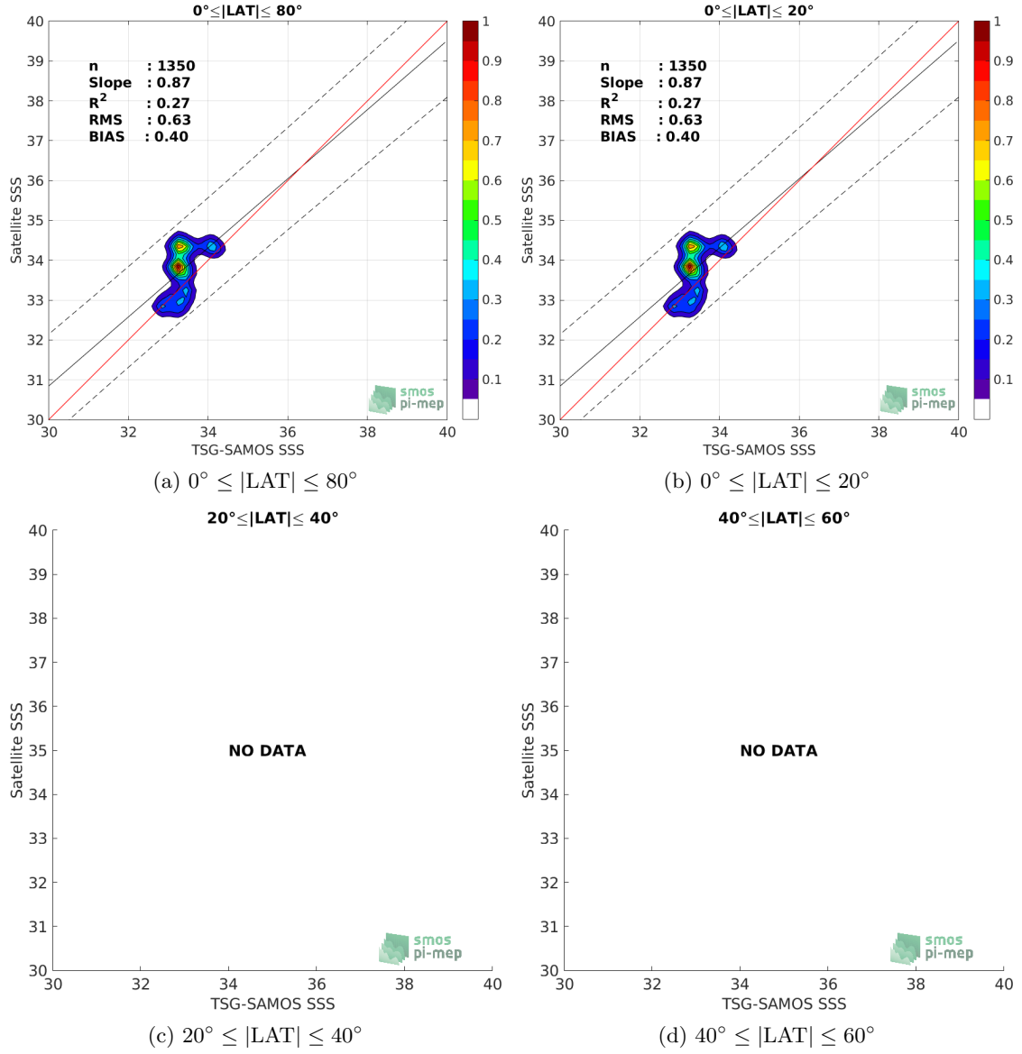
Figure 9: Contour maps of the concentration of SMOS-L3-CATDS-CECOS-LOCEAN-V4-18DAYS-25KM SSS (y-axis) versus TSG-SAMOS SSS (x-axis) at match-up pairs for different latitude bands. For each plot, the red line shows x=y . The black thin and dashed lines indicate a linear fit through the data cloud and the \pm 95\% confidence levels, respectively. The number match-up pairs n , the slope and R^2 coefficient of the linear fit, the root mean square (RMS) and the mean bias between satellite and in situ data are indicated for each latitude band in each plots.
