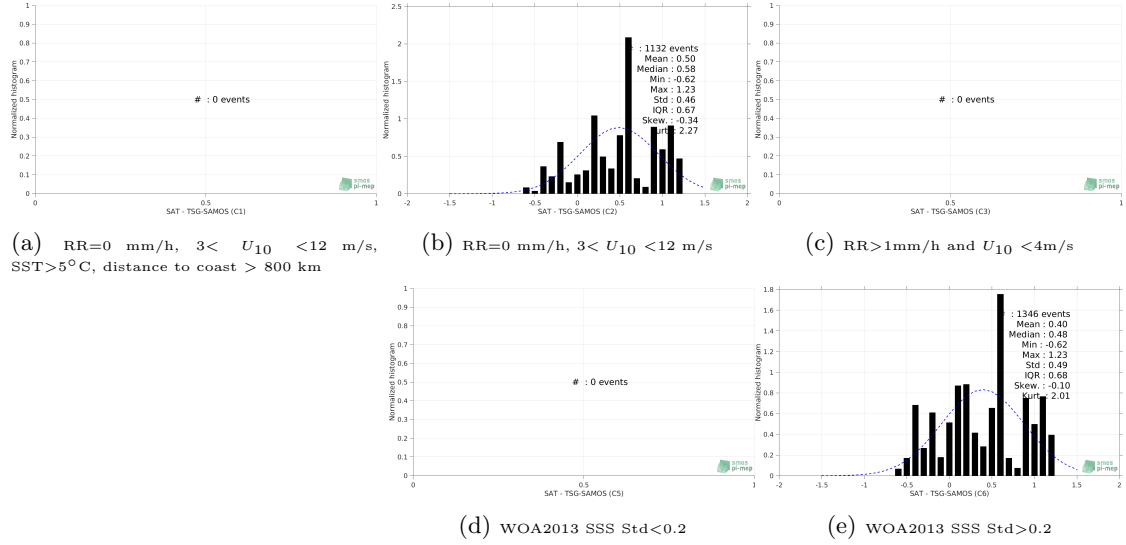
Figure 13: Normalized histogram of \Delta SSS (SMOS-L3-CATDS-CECOS-LOCEAN-V4-18DAYS-25KM - TSG-SAMOS) for 5 different subdatasets corresponding to: RR=0 mm/h, 3 < U_{10} < 12 m/s, SST>5°C, distance to coast > 800 km (a), RR=0 mm/h, 3 < U_{10} < 12 m/s (b), RR>1mm/h and U_{10} < 4 m/s (c), WOA2013 SSS Std<0.2 (d), WOA2013 SSS Std>0.2 (e).
