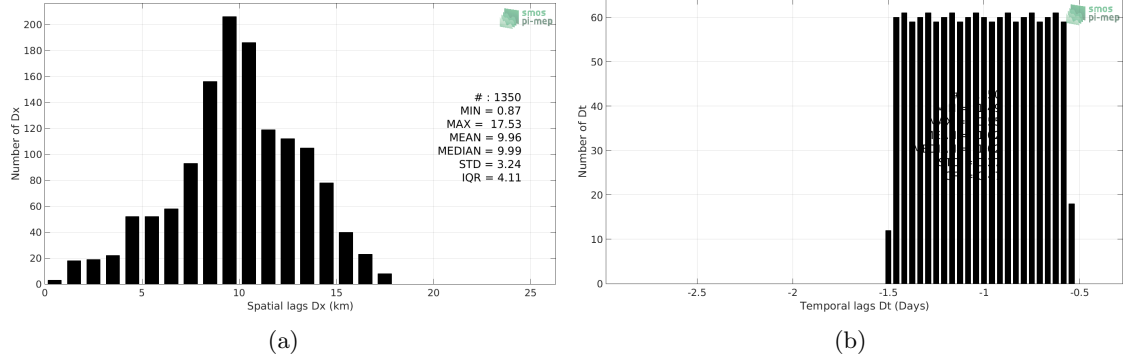
Figure 5: Histograms of the spatial (a) and temporal (b) lags between the time of the TSG-SAMOS measurements and the date of the corresponding SMOS-L3-CATDS-CECOS-LOCEAN-V4-18DAYS-25KM SSS product.
