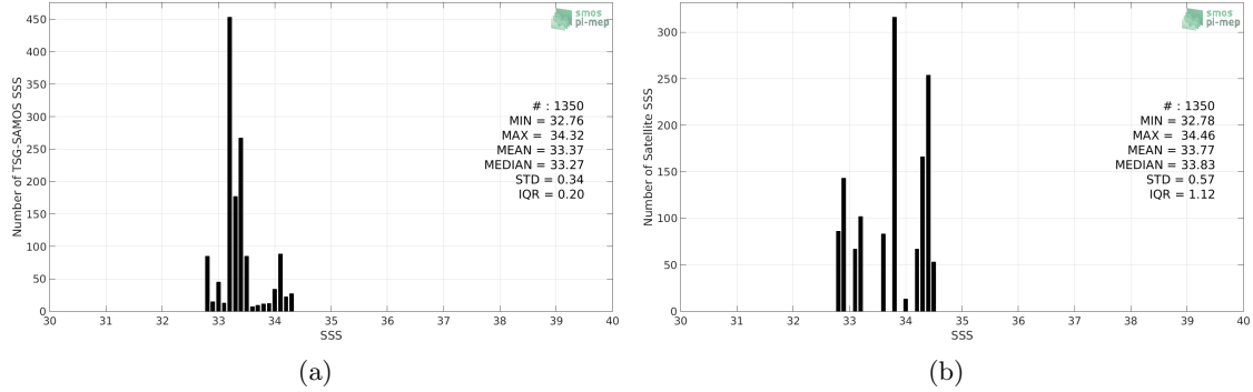
Figure 2: Histograms of SSS from TSG-SAMOS (a) and SMOS-L3-CATDS-CECOS-LOCEAN-V4-18DAYS-25KM (b) considering all match-up pairs per bins of 0.1 over the Ganga and Brahmaputra river plumes Pi-MEP region and for the full satellite product period.
