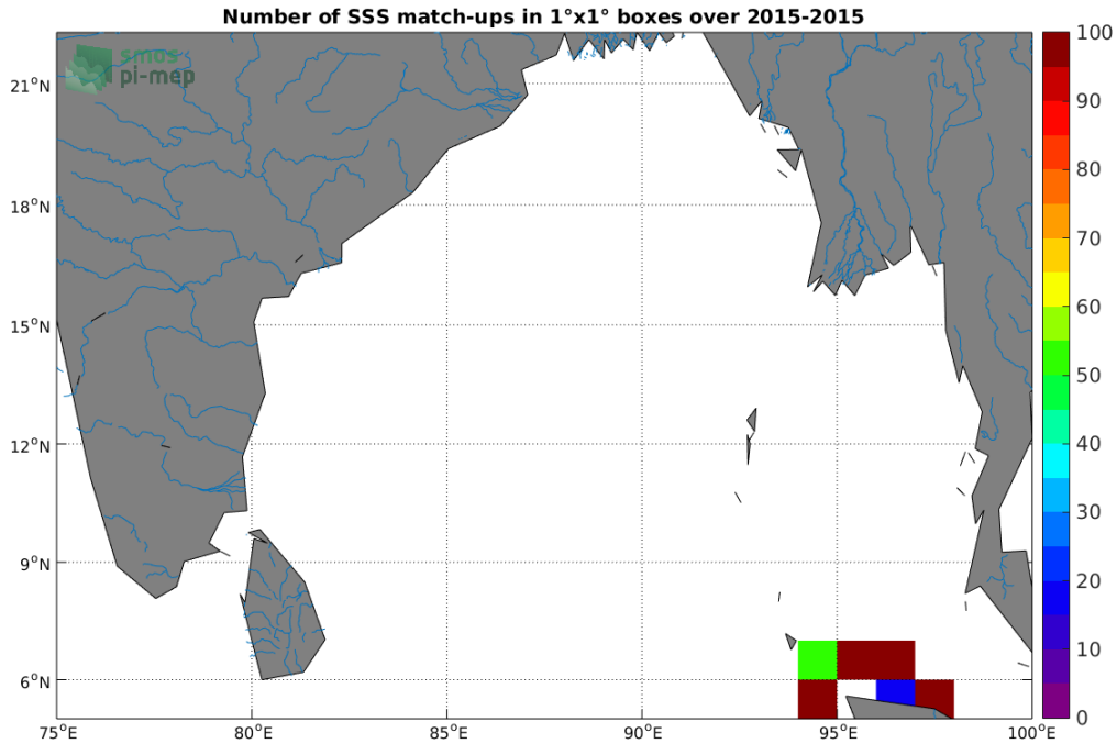
Figure 4: Number of SSS match-ups between TSG-SAMOS SSS and the SMOS-L3-CATDS-CECOS-LOCEAN-V4-18DAYS-25KM SSS product for the Ganga and Brahmaputra river plumes Pi-MEP region over 1°x1° boxes and for the full satellite product period.
