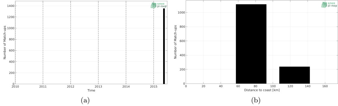
Figure 1: Number of match-ups between TSG-SAMOS and SMOS-L3-CATDS-CECOS-LOCEAN-V4-18DAYS-25KM SSS as a function of time (a) and as function of the distance to coast (b) over the Ganga and Brahmaputra river plumes Pi-MEP region and for the full satellite product period.
