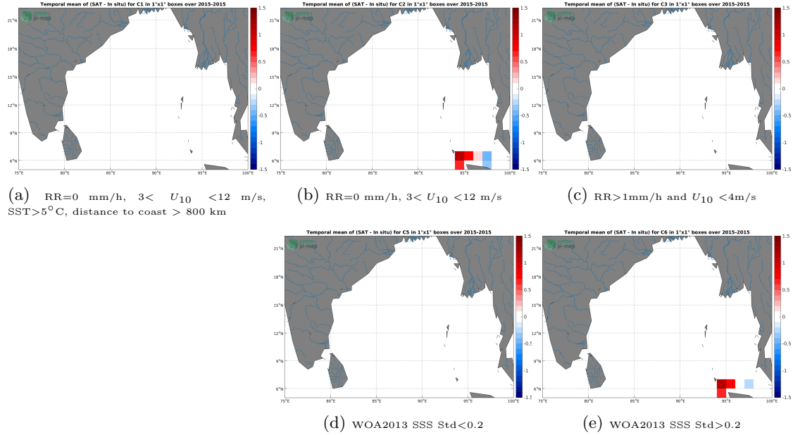
Figure 12: Temporal mean gridded over spatial boxes of size 1^{\circ}\times 1^{\circ} of \Delta\text{SSS} (SMOS-L3-CATDS-CECOS-LOCEAN-V4-18DAYS-25KM - TSG-SAMOS) for 5 different subdatasets corresponding to: RR=0 mm/h, 3 < U_{10} < 12 m/s, SST >5^{\circ}\text{C} , distance to coast > 800 km (a), RR=0 mm/h, 3 < U_{10} < 12 m/s (b), RR >1 mm/h and U_{10} < 4 m/s (c), WOA2013 SSS Std <0.2 (d), WOA2013 SSS Std >0.2 (e).
