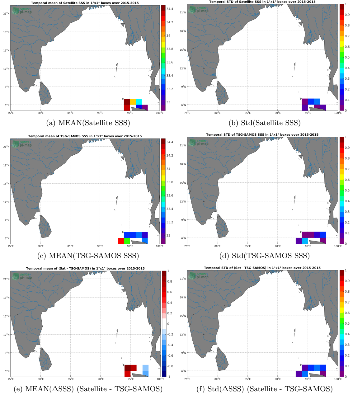
Figure 6: Temporal mean (left) and Std (right) of SSS from SMOS-L3-CATDS-CECOS-LOCEAN-V4-18DAYS-25KM (top), TSG-SAMOS (middle), and of \Delta SSS (Satellite - TSG-SAMOS). Only match-up pairs are used to generate these maps.
