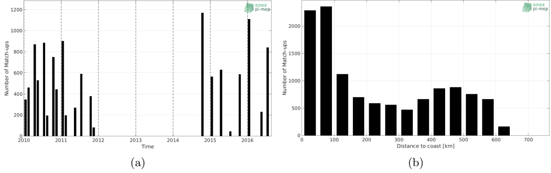
Figure 1: Number of match-ups between TSG (LEGOS-DM) and SMOS SSS L3 v4 - 18 Days (CATDS-CECOS-LOCEAN) SSS as a function of time (a) and as function of the distance to coast (b) over the Ganga and Brahmaputra river plumes Pi-MEP region and for the full satellite product period.
