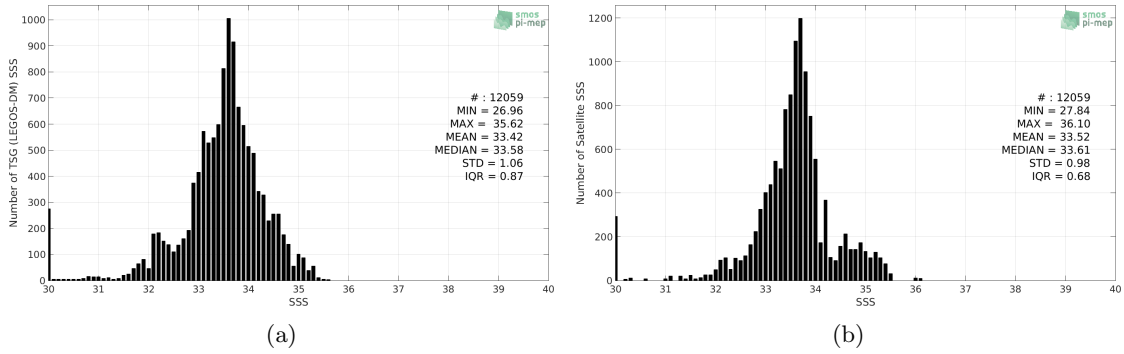
Figure 2: Histograms of SSS from TSG (LEGOS-DM) (a) and SMOS SSS L3 v4 - 18 Days (CATDS-CECOS-LOCEAN) (b) considering all match-up pairs per bins of 0.1 over the Ganga and Brahmaputra river plumes Pi-MEP region and for the full satellite product period.
