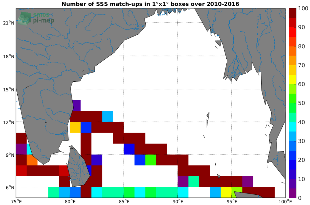
Figure 4: Number of SSS match-ups between TSG (LEGOS-DM) SSS and the SMOS SSS L3 v4 - 18 Days (CATDS-CECOS-LOCEAN) SSS product for the Ganga and Brahmaputra river plumes Pi-MEP region over 1°x1° boxes and for the full satellite product period.
