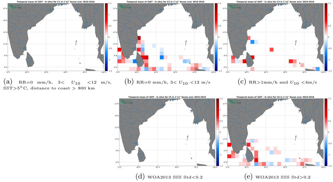
Figure 12: Temporal mean gridded over spatial boxes of size 1^{\circ}\times 1^{\circ} of \Delta\text{SSS} (SMOS SSS L3 v4 - 18 Days (CATDS-CECOS-LOCEAN) - TSG (LEGOS-DM)) for 5 different subdatasets corresponding to:RR=0 mm/h, 3 < U_{10} < 12 m/s, SST >5^{\circ}\text{C} , distance to coast > 800 km (a), RR=0 mm/h, 3 < U_{10} < 12 m/s (b), RR >1 mm/h and U_{10} < 4 m/s (c), WOA2013 SSS Std <0.2 (d), WOA2013 SSS Std >0.2 (e).
