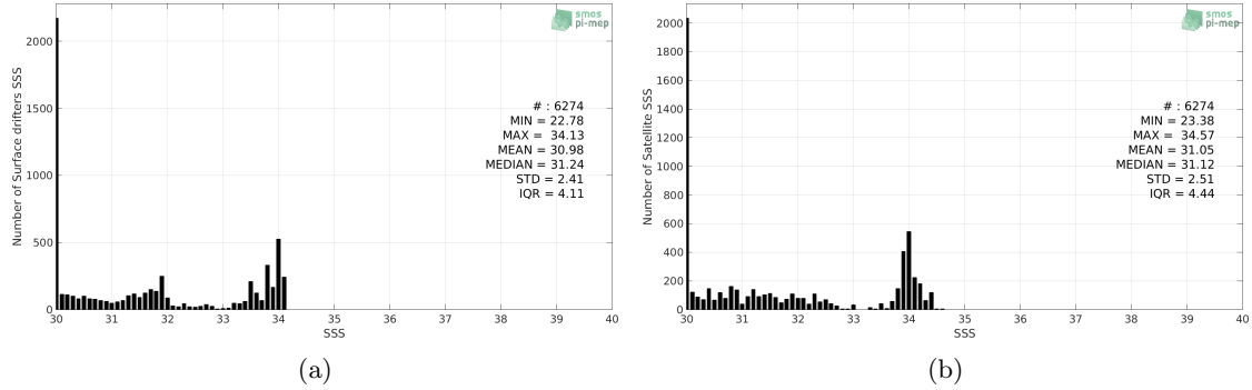
Figure 2: Histograms of SSS from Surface drifters (a) and SMOS-L3-CATDS-CECOS-LOCEAN-V4-18DAYS-25KM (b) considering all match-up pairs per bins of 0.1 over the Ganga and Brahmaputra river plumes Pi-MEP region and for the full satellite product period.
