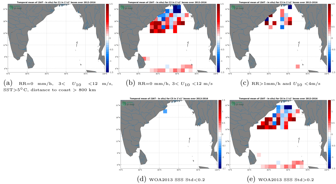
Figure 11: Temporal mean gridded over spatial boxes of size 1^{\circ}\times 1^{\circ} of \Delta\text{SSS} (SMOS-L3-CATDS-CECOS-LOCEAN-V4-18DAYS-25KM - Surface drifters) for 5 different subdatasets corresponding to: RR=0 mm/h, 3 < U_{10} < 12 m/s, SST >5^{\circ}\text{C} , distance to coast > 800 km (a), RR=0 mm/h, 3 < U_{10} < 12 m/s (b), RR >1 mm/h and U_{10} < 4 m/s (c), WOA2013 SSS Std <0.2 (d), WOA2013 SSS Std >0.2 (e).
