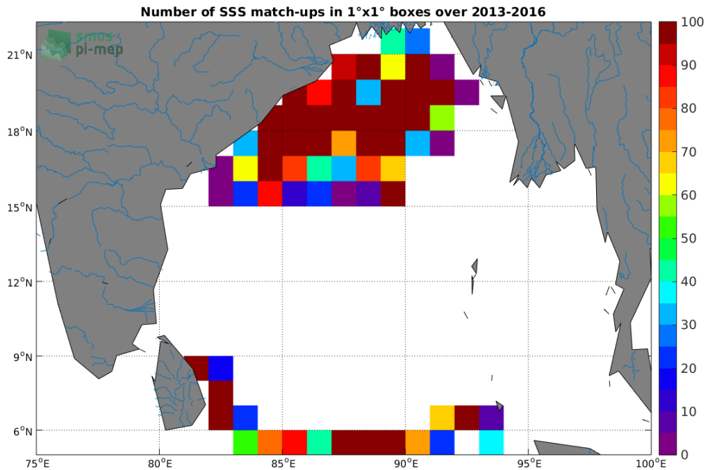
Figure 3: Number of SSS match-ups between Surface drifters SSS and the SMOS-L3-CATDS-CECOS-LOCEAN-V4-18DAYS-25KM SSS product for the Ganga and Brahmaputra river plumes Pi-MEP region over 1^\circ \times 1^\circ boxes and for the full satellite product period.
