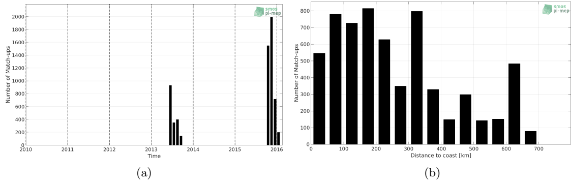
Figure 1: Number of match-ups between Surface drifters and SMOS-L3-CATDS-CECOS-LOCEAN-V4-18DAYS-25KM SSS as a function of time (a) and as function of the distance to coast (b) over the Ganga and Brahmaputra river plumes Pi-MEP region and for the full satellite product period.
