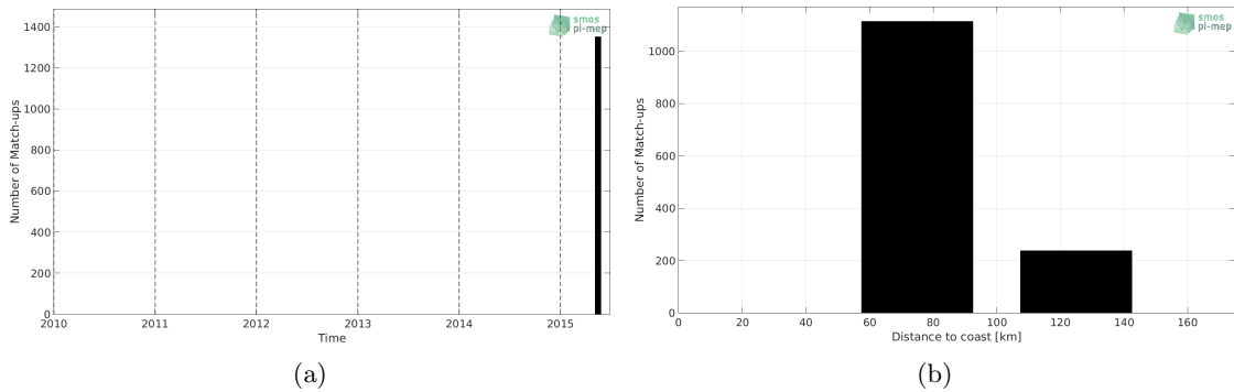
Figure 1: Number of match-ups between TSG-SAMOS and SMOS-L3-CATDS-CECOS-LOCEAN-V3-9DAYS-25KM SSS as a function of time (a) and as function of the distance to coast (b) over the Ganga and Brahmaputra river plumes Pi-MEP region and for the full satellite product period.
