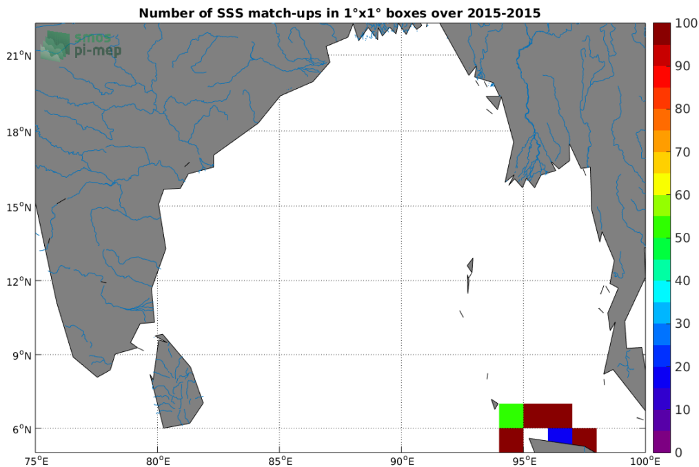
Figure 4: Number of SSS match-ups between TSG-SAMOS SSS and the SMOS-L3-CATDS-CECOS-LOCEAN-V3-9DAYS-25KM SSS product for the Ganga and Brahmaputra river plumes Pi-MEP region over 1^{\circ} \times 1^{\circ} boxes and for the full satellite product period.
