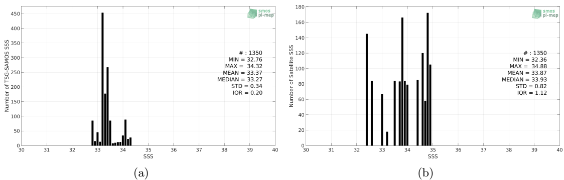
Figure 2: Histograms of SSS from TSG-SAMOS (a) and SMOS-L3-CATDS-CECOS-LOCEAN-V3-9DAYS-25KM (b) considering all match-up pairs per bins of 0.1 over the Ganga and Brahmaputra river plumes Pi-MEP region and for the full satellite product period.
