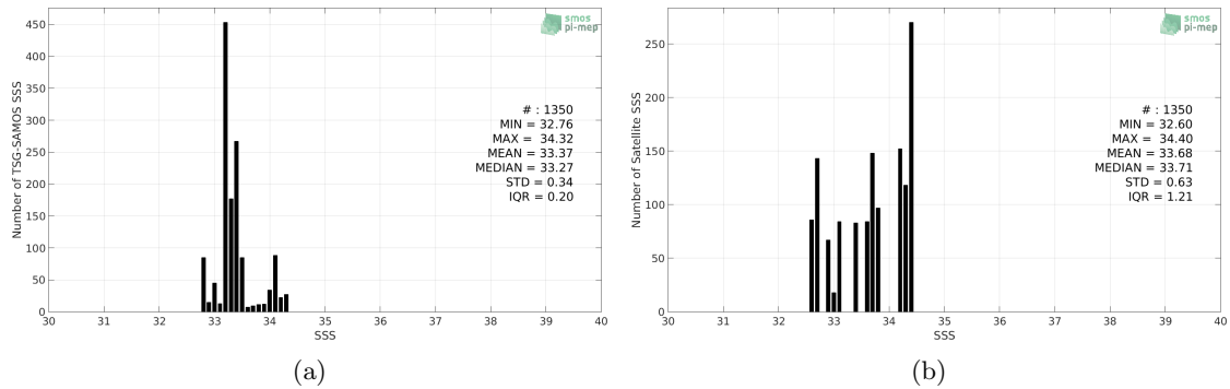
Figure 2: Histograms of SSS from TSG-SAMOS (a) and SMOS-L3-CATDS-CECOS-LOCEAN-V3-18DAYS-25KM (b) considering all match-up pairs per bins of 0.1 over the Ganga and Brahmaputra river plumes Pi-MEP region and for the full satellite product period.
