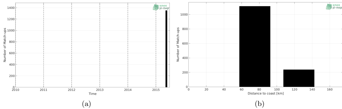
Figure 1: Number of match-ups between TSG-SAMOS and SMOS-L3-CATDS-CECOS-LOCEAN-V3-18DAYS-25KM SSS as a function of time (a) and as function of the distance to coast (b) over the Ganga and Brahmaputra river plumes Pi-MEP region and for the full satellite product period.
