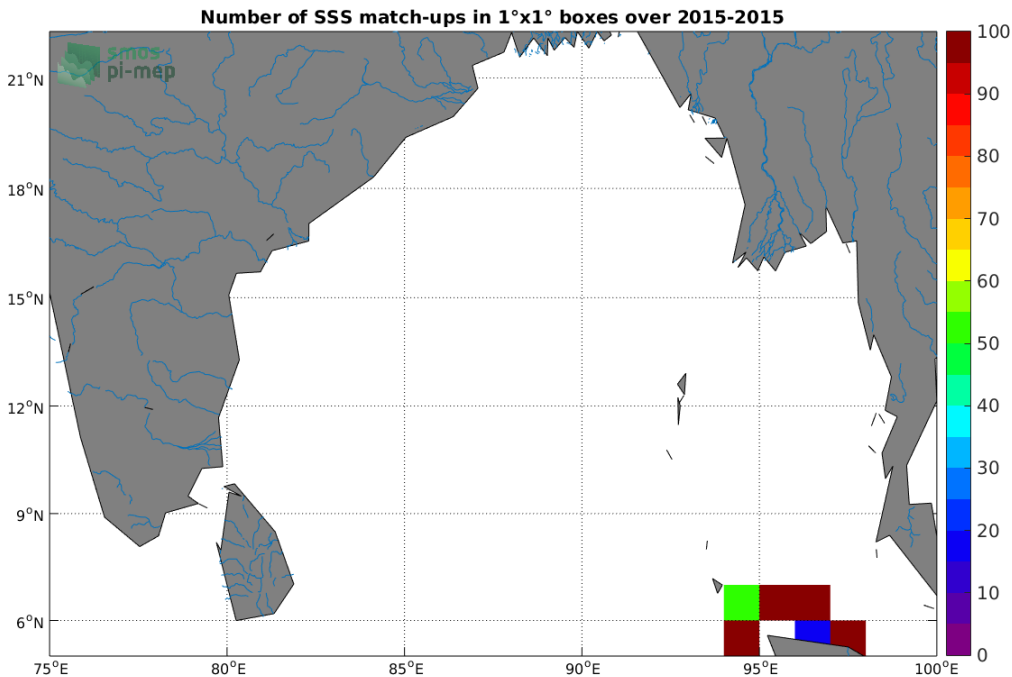
Figure 4: Number of SSS match-ups between TSG-SAMOS SSS and the SMOS-L3-CATDS-CECOS-LOCEAN-V3-18DAYS-25KM SSS product for the Ganga and Brahmaputra river plumes Pi-MEP region over 1°x1° boxes and for the full satellite product period.
