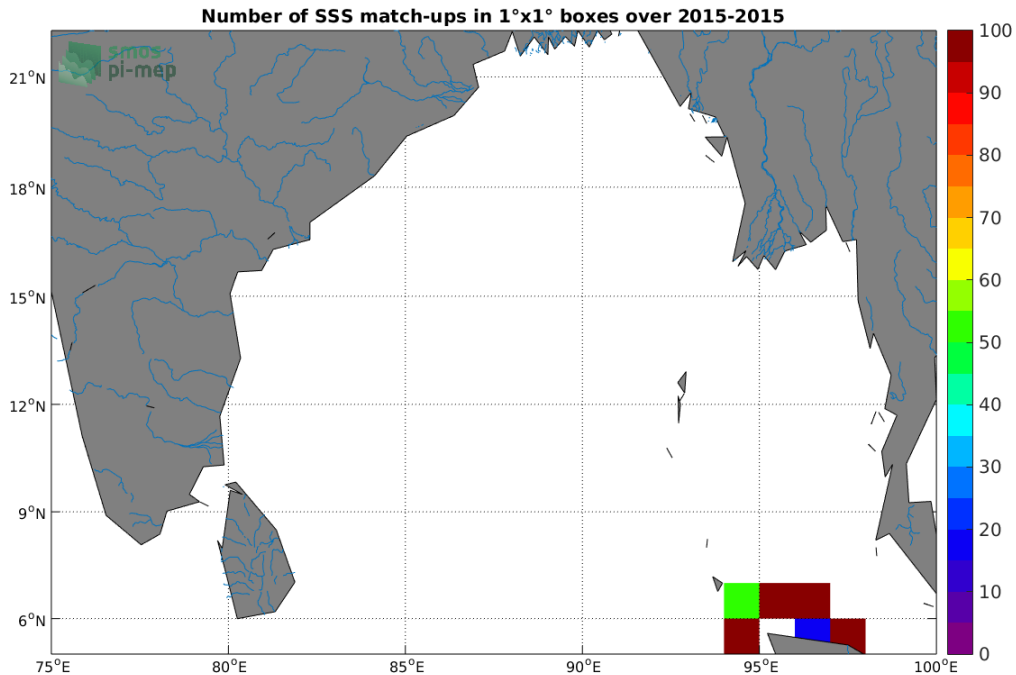
Figure 4: Number of SSS match-ups between TSG-SAMOS SSS and the SMOS-L3-CATDS-CECOS-LOCEAN-V3-18DAYS-25KM SSS product for the Ganga and Brahmaputra river plumes Pi-MEP region over 1^{\circ} \times 1^{\circ} boxes and for the full satellite product period.
