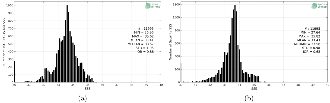
Figure 2: Histograms of SSS from TSG-LEGOS-DM (a) and SMOS-L3-CATDS-CECOS-LOCEAN-V3-18DAYS-25KM (b) considering all match-up pairs per bins of 0.1 over the Ganga and Brahmaputra river plumes Pi-MEP region and for the full satellite product period.
