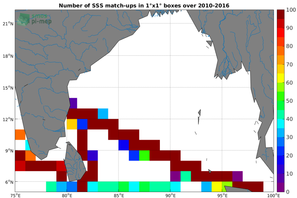
Figure 4: Number of SSS match-ups between TSG-LEGOS-DM SSS and the SMOS-L3-CATDS-CECOS-LOCEAN-V3-18DAYS-25KM SSS product for the Ganga and Brahmaputra river plumes Pi-MEP region over 1^\circ \times 1^\circ boxes and for the full satellite product period.
