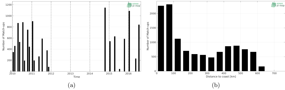
Figure 1: Number of match-ups between TSG-LEGOS-DM and SMOS-L3-CATDS-CECOS-LOCEAN-V3-18DAYS-25KM SSS as a function of time (a) and as function of the distance to coast (b) over the Ganga and Brahmaputra river plumes Pi-MEP region and for the full satellite product period.
