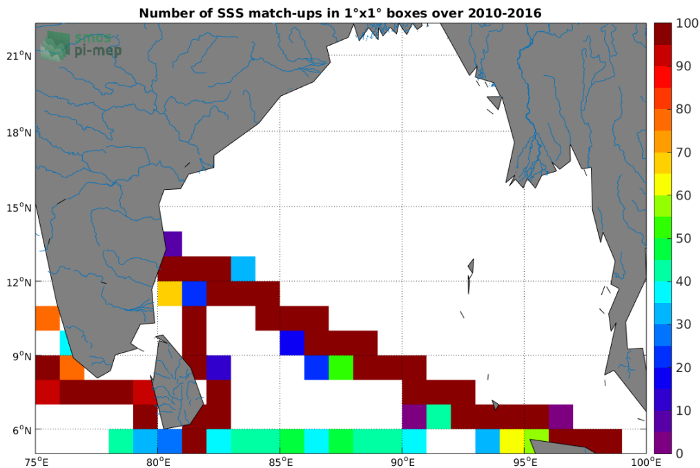
Figure 4: Number of SSS match-ups between TSG-LEGOS-DM SSS and the SMOS-L3-CATDS-CECOS-LOCEAN-V3-18DAYS-25KM SSS product for the Ganga and Brahmaputra river plumes Pi-MEP region over 1^{\circ} \times 1^{\circ} boxes and for the full satellite product period.
