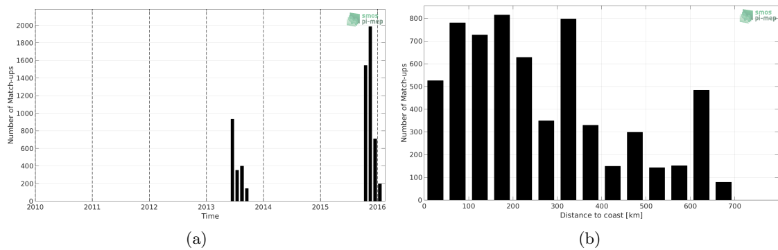
Figure 1: Number of match-ups between Surface drifters and SMOS-L3-CATDS-CECOS-LOCEAN-V3-18DAYS-25KM SSS as a function of time (a) and as function of the distance to coast (b) over the Ganga and Brahmaputra river plumes Pi-MEP region and for the full satellite product period.
