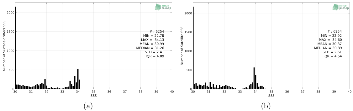
Figure 2: Histograms of SSS from Surface drifters (a) and SMOS-L3-CATDS-CECOS-LOCEAN-V3-18DAYS-25KM (b) considering all match-up pairs per bins of 0.1 over the Ganga and Brahmaputra river plumes Pi-MEP region and for the full satellite product period.
