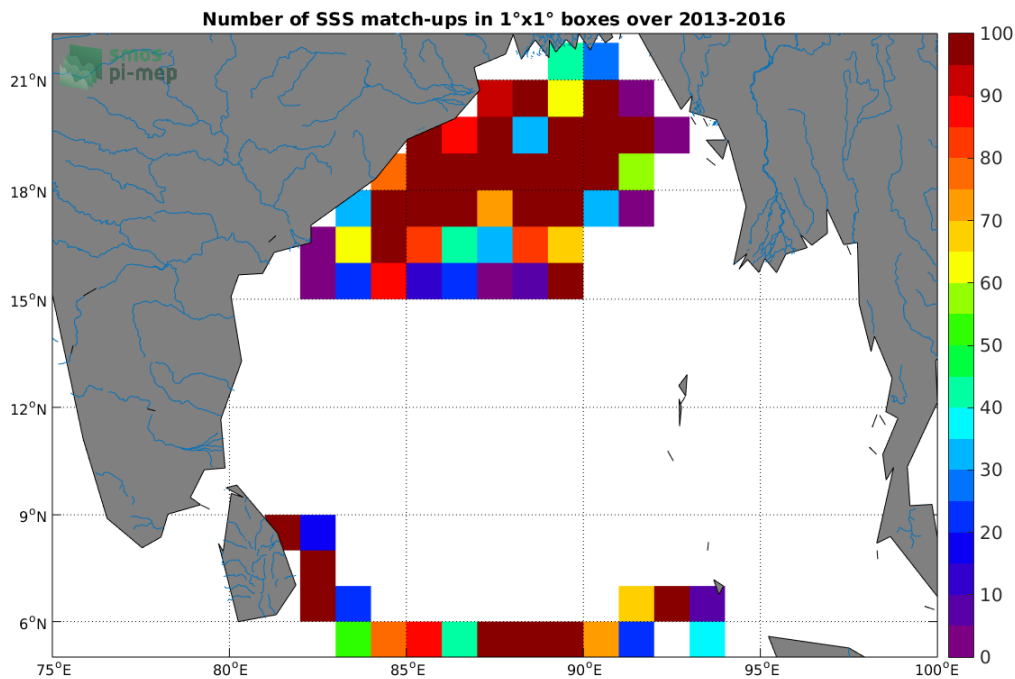
Figure 3: Number of SSS match-ups between Surface drifters SSS and the SMOS-L3-CATDS-CECOS-LOCEAN-V3-18DAYS-25KM SSS product for the Ganga and Brahmaputra river plumes Pi-MEP region over 1^{\circ} \times 1^{\circ} boxes and for the full satellite product period.
