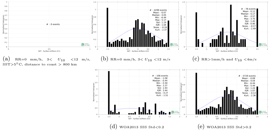
Figure 12: Normalized histogram of \Delta SSS (SMOS-L3-CATDS-CECOS-LOCEAN-V3-18DAYS-25KM - Surface drifters) for 5 different subdatasets corresponding to: RR=0 mm/h, 3 < U_{10} < 12 m/s, SST > 5°C, distance to coast > 800 km (a), RR=0 mm/h, 3 < U_{10} < 12 m/s (b), RR > 1mm/h and U_{10} < 4 m/s (c), WOA2013 SSS Std < 0.2 (d), WOA2013 SSS Std > 0.2 (e).
