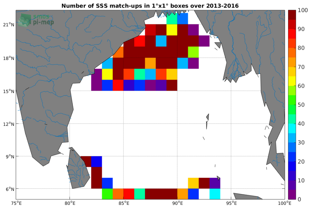
Figure 3: Number of SSS match-ups between Surface drifters SSS and the SMOS-L3-CATDS-CECOS-LOCEAN-V3-18DAYS-25KM SSS product for the Ganga and Brahmaputra river plumes Pi-MEP region over 1°x1° boxes and for the full satellite product period.
