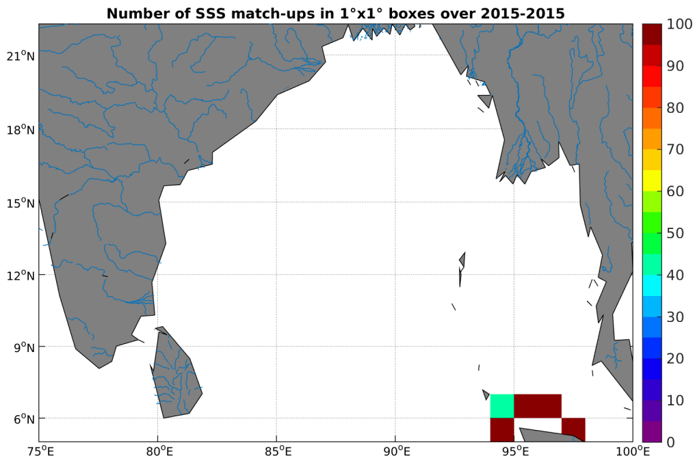
Figure 4: Number of SSS match-ups between TSG-SAMOS SSS and the SMOS-L3-CATDS-CECOS-LOCEAN-V2.1-9DAYS-25KM SSS product for the Ganga and Brahmaputra river plumes Pi-MEP region over 1°x1° boxes and for the full satellite product period.
