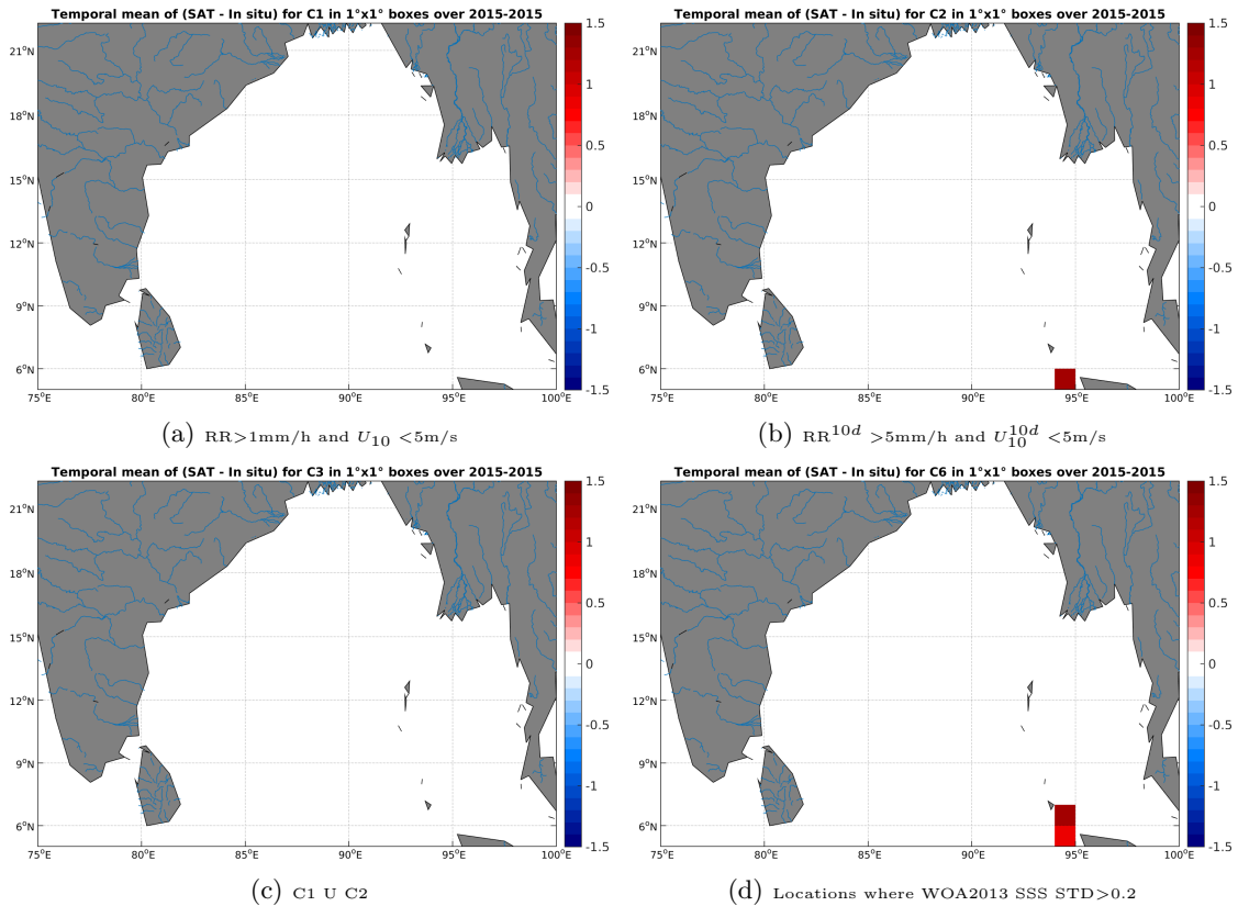
Figure 12: Temporal mean gridded over spatial boxes of size 1°x1° of \Delta SSS (SMOS-L3-CATDS-CECOS-LOCEAN-V2.1-9DAYS-25KM - TSG-SAMOS) for 4 different subdatasets corresponding to: RR > 1mm/h and U_{10} < 5\text{m/s} (a), RR^{10d} > 5\text{mm/h} and U_{10}^{10d} < 5\text{m/s} (b), C1 U C2 (c), Locations where WOA2013 SSS STD > 0.2 (d).
