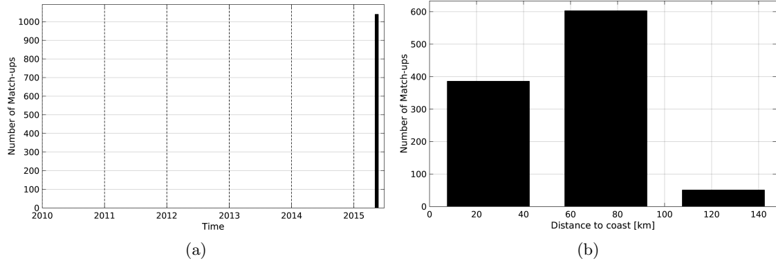
Figure 1: Number of match-ups between TSG-SAMOS and SMOS-L3-CATDS-CECOS-LOCEAN-V2.1-9DAYS-25KM SSS as a function of time (a) and as function of the distance to coast (b) over the Ganga and Brahmaputra river plumes Pi-MEP region and for the full satellite product period.
