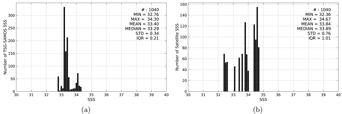
Figure 2: Histograms of SSS from TSG-SAMOS (a) and SMOS-L3-CATDS-CECOS-LOCEAN-V2.1-9DAYS-25KM (b) considering all match-up pairs per bins of 0.1 over the Ganga and Brahmaputra river plumes Pi-MEP region and for the full satellite product period.
