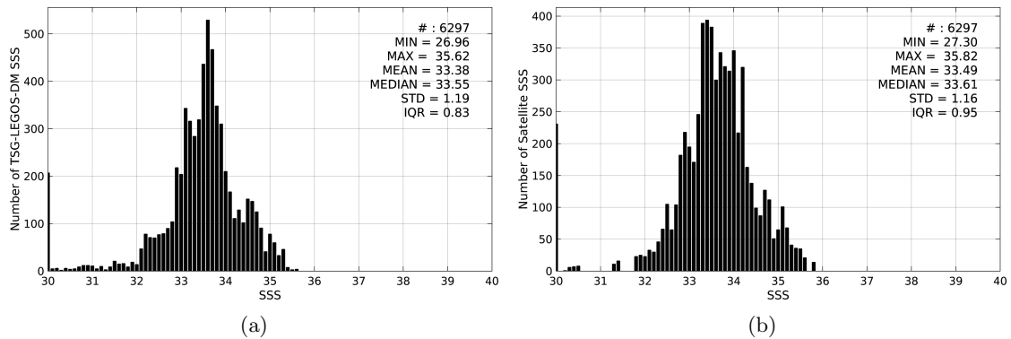
Figure 2: Histograms of SSS from TSG-LEGOS-DM (a) and SMOS-L3-CATDS-CECOS-LOCEAN-V2.1-9DAYS-25KM (b) considering all match-up pairs per bins of 0.1 over the Ganga and Brahmaputra river plumes Pi-MEP region and for the full satellite product period.
