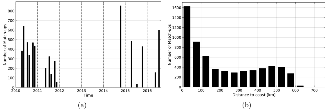
Figure 1: Number of match-ups between TSG-LEGOS-DM and SMOS-L3-CATDS-CECOS-LOCEAN-V2.1-9DAYS-25KM SSS as a function of time (a) and as function of the distance to coast (b) over the Ganga and Brahmaputra river plumes Pi-MEP region and for the full satellite product period.
