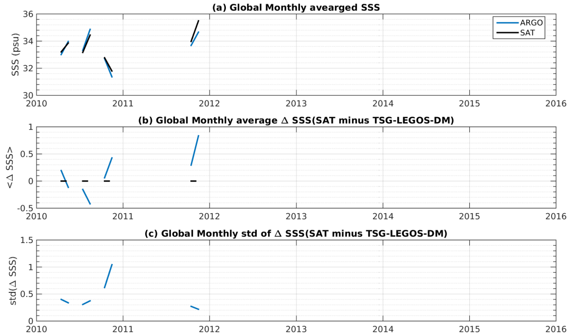
Figure 7: Time series of the monthly averaged mean SSS (top), mean \Delta SSS (Satellite - TSG-LEGOS-DM) and STD of \Delta SSS (Satellite - TSG-LEGOS-DM) over the Ganga and Brahmaputra river plumes Pi-MEP region considering all match-ups collected by the Pi-MEP platform.
