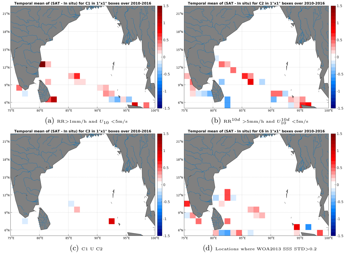
Figure 12: Temporal mean gridded over spatial boxes of size 1°x1° of \Delta SSS (SMOS-L3-CATDS-CECOS-LOCEAN-V2.1-9DAYS-25KM - TSG-LEGOS-DM) for 4 different subdatasets corresponding to:RR>1mm/h and U_{10} < 5 m/s (a), RR^{10d} > 5 mm/h and U_{10}^{10d} < 5 m/s (b), C1 U C2 (c),Locations where WOA2013 SSS STD>0.2 (d).
