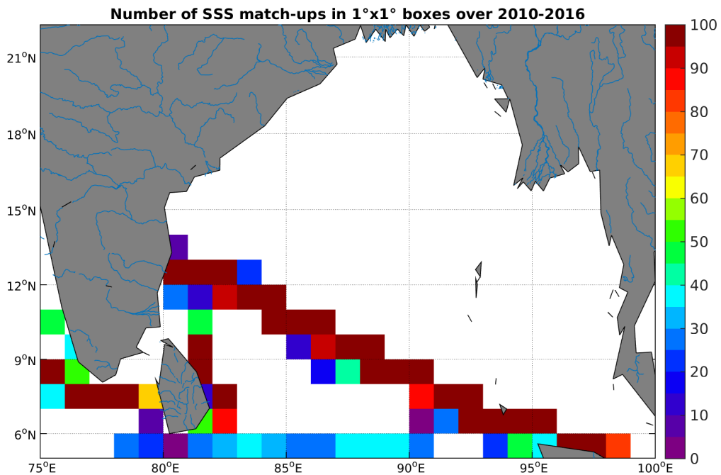
Figure 4: Number of SSS match-ups between TSG-LEGOS-DM SSS and the SMOS-L3-CATDS-CECOS-LOCEAN-V2.1-9DAYS-25KM SSS product for the Ganga and Brahmaputra river plumes Pi-MEP region over 1°x1° boxes and for the full satellite product period.
