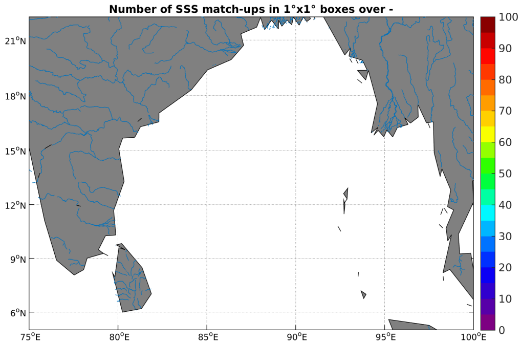
Figure 4: Number of SSS match-ups between TSG-GOSUD-Sailing-ship SSS and the SMOS-L3-CATDS-CECOS-LOCEAN-V2.1-9DAYS-25KM SSS product for the Ganga and Brahmaputra river plumes Pi-MEP region over 1°x1° boxes and for the full satellite product period.
