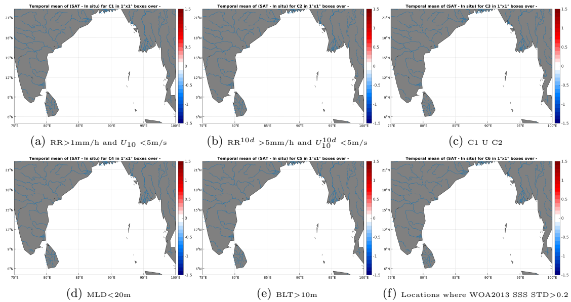
Figure 12: Temporal mean gridded over spatial boxes of size 1^\circ \times 1^\circ of \Delta SSS (SMOS-L3-CATDS-CECOS-LOCEAN-V2.1-9DAYS-25KM - Sea mammals) for 6 different subdatasets corresponding to:RR >1 mm/h and U_{10} < 5 m/s (a), RR ^{10d} > 5 mm/h and U_{10}^{10d} < 5 m/s (b), C1 U C2 (c),MLD <20 m (d),BLT >10 m (e),Locations where WOA2013 SSS STD >0.2 (f).
