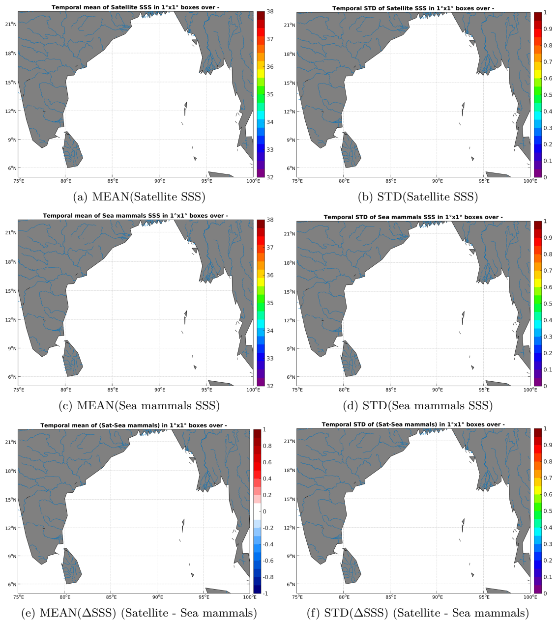
Figure 6: Temporal mean (left) and STD (right) of SSS from SMOS-L3-CATDS-CECOS-LOCEAN-V2.1-9DAYS-25KM (top), Sea mammals (middle), and of \Delta SSS (Satellite - Sea mammals). Only match-up pairs are used to generate these maps.
