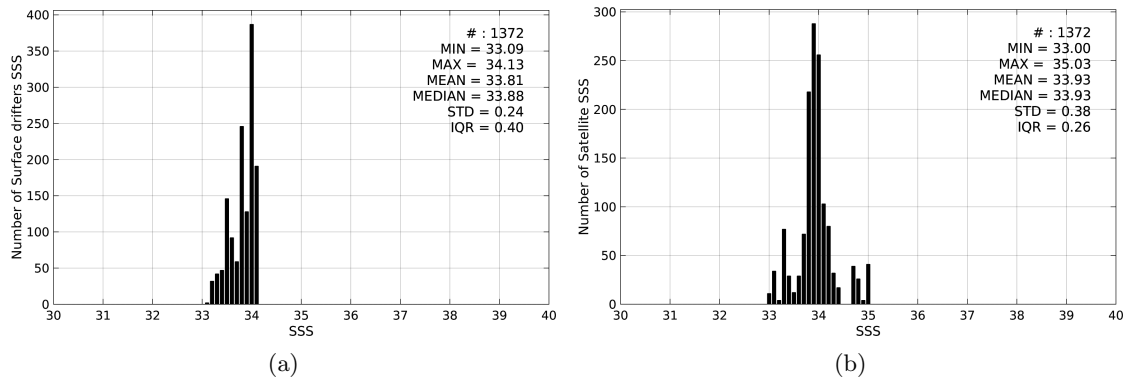
Figure 2: Histograms of SSS from Surface drifters (a) and SMOS-L3-CATDS-CECOS-LOCEAN-V2.1-9DAYS-25KM (b) considering all match-up pairs per bins of 0.1 over the Ganga and Brahmaputra river plumes Pi-MEP region and for the full satellite product period.
