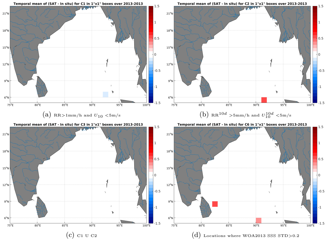
Figure 11: Temporal mean gridded over spatial boxes of size 1°x1° of \Delta SSS (SMOS-L3-CATDS-CECOS-LOCEAN-V2.1-9DAYS-25KM - Surface drifters) for 4 different subdatasets corresponding to: RR > 1mm/h and U_{10} < 5\text{m/s} (a), RR^{10d} > 5\text{mm/h} and U_{10}^{10d} < 5\text{m/s} (b), C1 U C2 (c), Locations where WOA2013 SSS STD > 0.2 (d).
