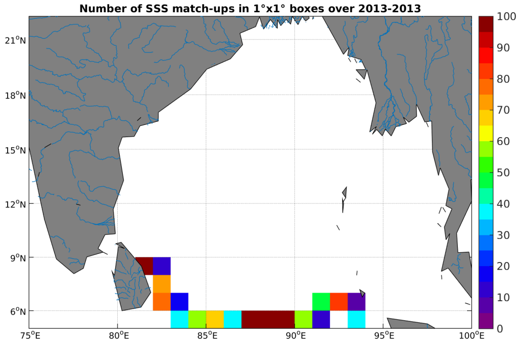
Figure 3: Number of SSS match-ups between Surface drifters SSS and the SMOS-L3-CATDS-CECOS-LOCEAN-V2.1-9DAYS-25KM SSS product for the Ganga and Brahmaputra river plumes Pi-MEP region over 1°x1° boxes and for the full satellite product period.
