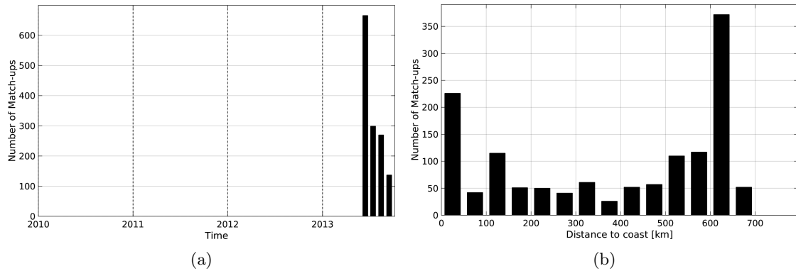
Figure 1: Number of match-ups between Surface drifters and SMOS-L3-CATDS-CECOS-LOCEAN-V2.1-9DAYS-25KM SSS as a function of time (a) and as function of the distance to coast (b) over the Ganga and Brahmaputra river plumes Pi-MEP region and for the full satellite product period.
