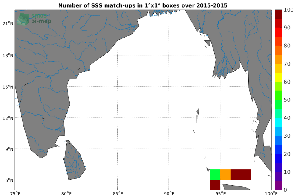
Figure 4: Number of SSS match-ups between TSG-SAMOS SSS and the SMOS L3 v2 - Monthly - 0.25 Deg (CATDS-CECOS-IFREMER) SSS product for the Ganga and Brahmaputra river plumes Pi-MEP region over 1^\circ \times 1^\circ boxes and for the full satellite product period.
