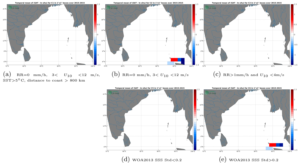
Figure 12: Temporal mean gridded over spatial boxes of size 1^{\circ}\times 1^{\circ} of \Delta\text{SSS} (SMOS L3 v2 - Monthly - 0.25 Deg (CATDS-CECOS-IFREMER) - TSG-SAMOS) for 5 different subdatasets corresponding to:RR=0 mm/h, 3 < U_{10} < 12 m/s, SST >5^{\circ}\text{C} , distance to coast > 800 km (a), RR=0 mm/h, 3 < U_{10} < 12 m/s (b), RR >1 mm/h and U_{10} < 4 m/s (c), WOA2013 SSS Std <0.2 (d), WOA2013 SSS Std >0.2 (e).
