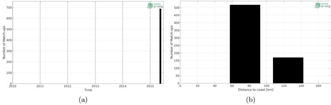
Figure 1: Number of match-ups between TSG-SAMOS and SMOS L3 v2 - Monthly - 0.25 Deg (CATDS-CECOS-IFREMER) SSS as a function of time (a) and as function of the distance to coast (b) over the Ganga and Brahmaputra river plumes Pi-MEP region and for the full satellite product period.
