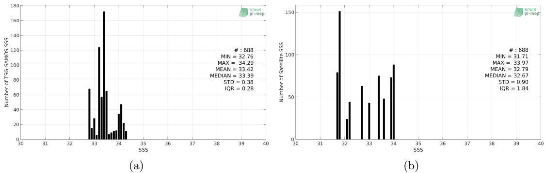
Figure 2: Histograms of SSS from TSG-SAMOS (a) and SMOS L3 v2 - Monthly - 0.25 Deg (CATDS-CECOS-IFREMER) (b) considering all match-up pairs per bins of 0.1 over the Ganga and Brahmaputra river plumes Pi-MEP region and for the full satellite product period.
