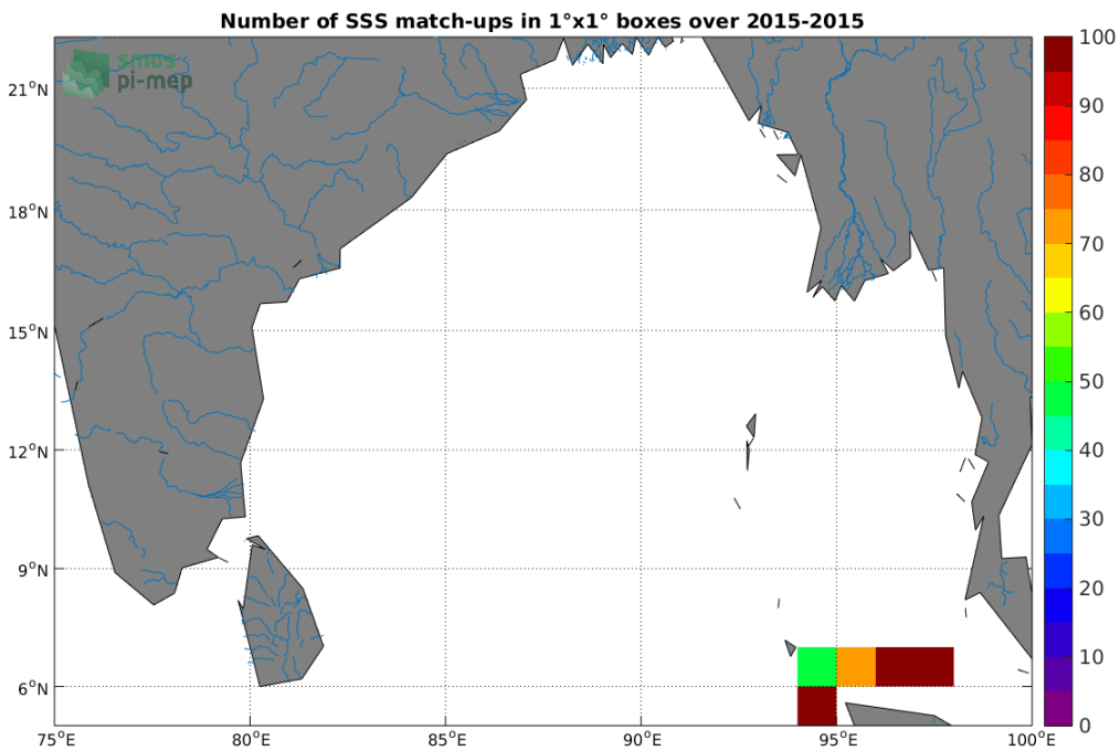
Figure 4: Number of SSS match-ups between TSG-SAMOS SSS and the SMOS-L3-CATDS-IFREMER-CECOS-V2-MONTHLY-0.25DEG SSS product for the Ganga and Brahmaputra river plumes Pi-MEP region over 1°x1° boxes and for the full satellite product period.
