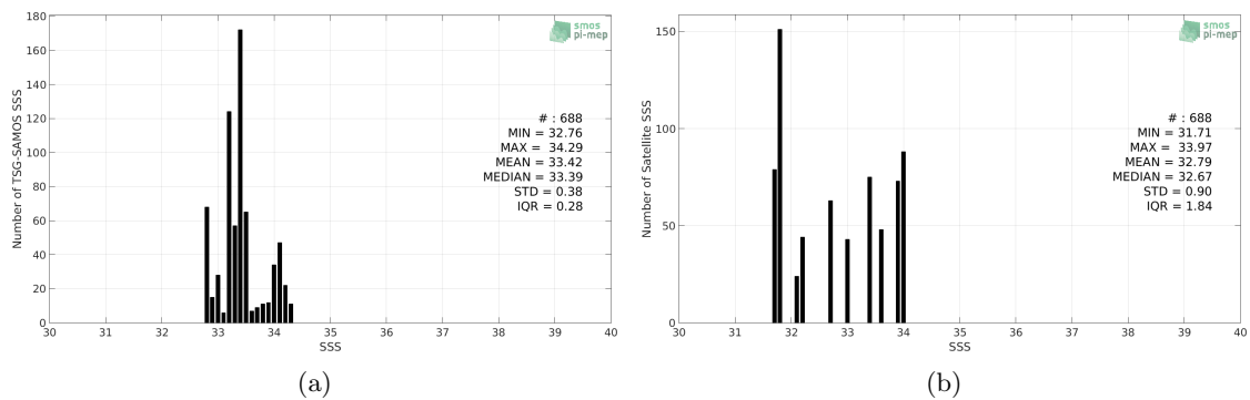
Figure 2: Histograms of SSS from TSG-SAMOS (a) and SMOS-L3-CATDS-IFREMER-CECOS-V2-MONTHLY-0.25DEG (b) considering all match-up pairs per bins of 0.1 over the Ganga and Brahmaputra river plumes Pi-MEP region and for the full satellite product period.
