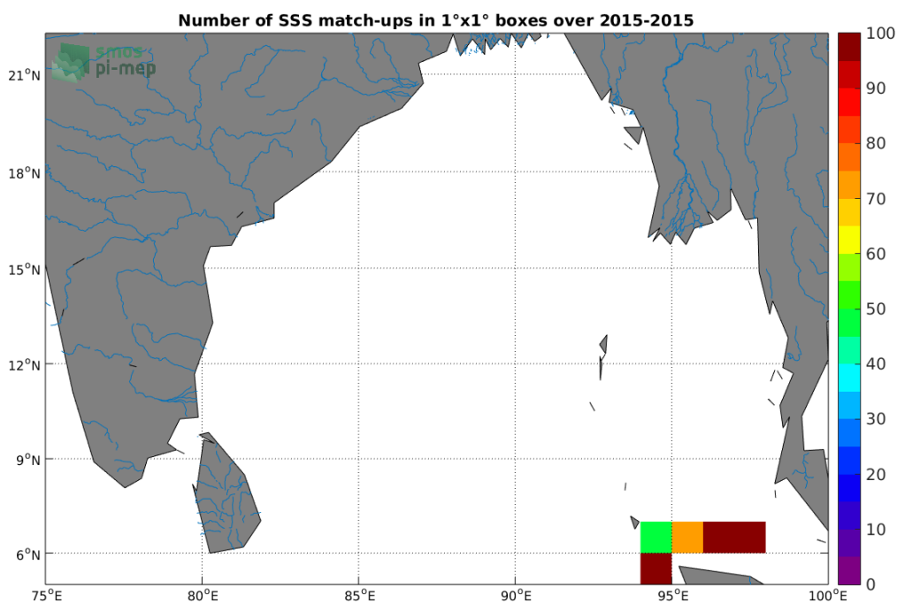
Figure 4: Number of SSS match-ups between TSG-SAMOS SSS and the SMOS-L3-CATDS-IFREMER-CECOS-V2-MONTHLY-0.25DEG SSS product for the Ganga and Brahmaputra river plumes Pi-MEP region over 1^\circ \times 1^\circ boxes and for the full satellite product period.
