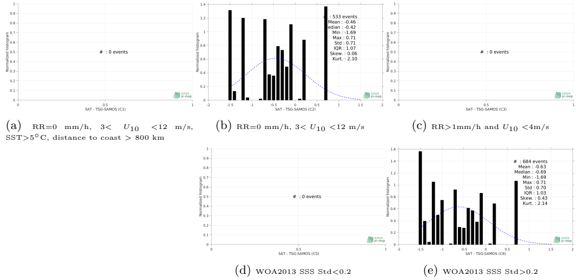
Figure 13: Normalized histogram of \Delta SSS (SMOS-L3-CATDS-IFREMER-CECOS-V2-MONTHLY-0.25DEG - TSG-SAMOS) for 5 different subdatasets corresponding to: RR=0 mm/h, 3 < U_{10} < 12 m/s, SST>5°C, distance to coast > 800 km (a), RR=0 mm/h, 3 < U_{10} < 12 m/s (b), RR>1mm/h and U_{10} < 4 m/s (c), WOA2013 SSS Std<0.2 (d), WOA2013 SSS Std>0.2 (e).
