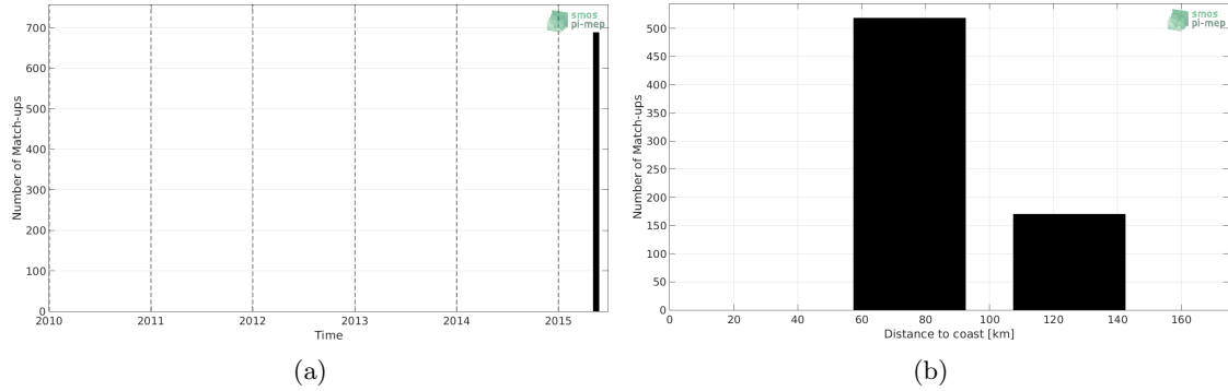
Figure 1: Number of match-ups between TSG-SAMOS and SMOS-L3-CATDS-IFREMER-CECOS-V2-MONTHLY-0.25DEG SSS as a function of time (a) and as function of the distance to coast (b) over the Ganga and Brahmaputra river plumes Pi-MEP region and for the full satellite product period.
